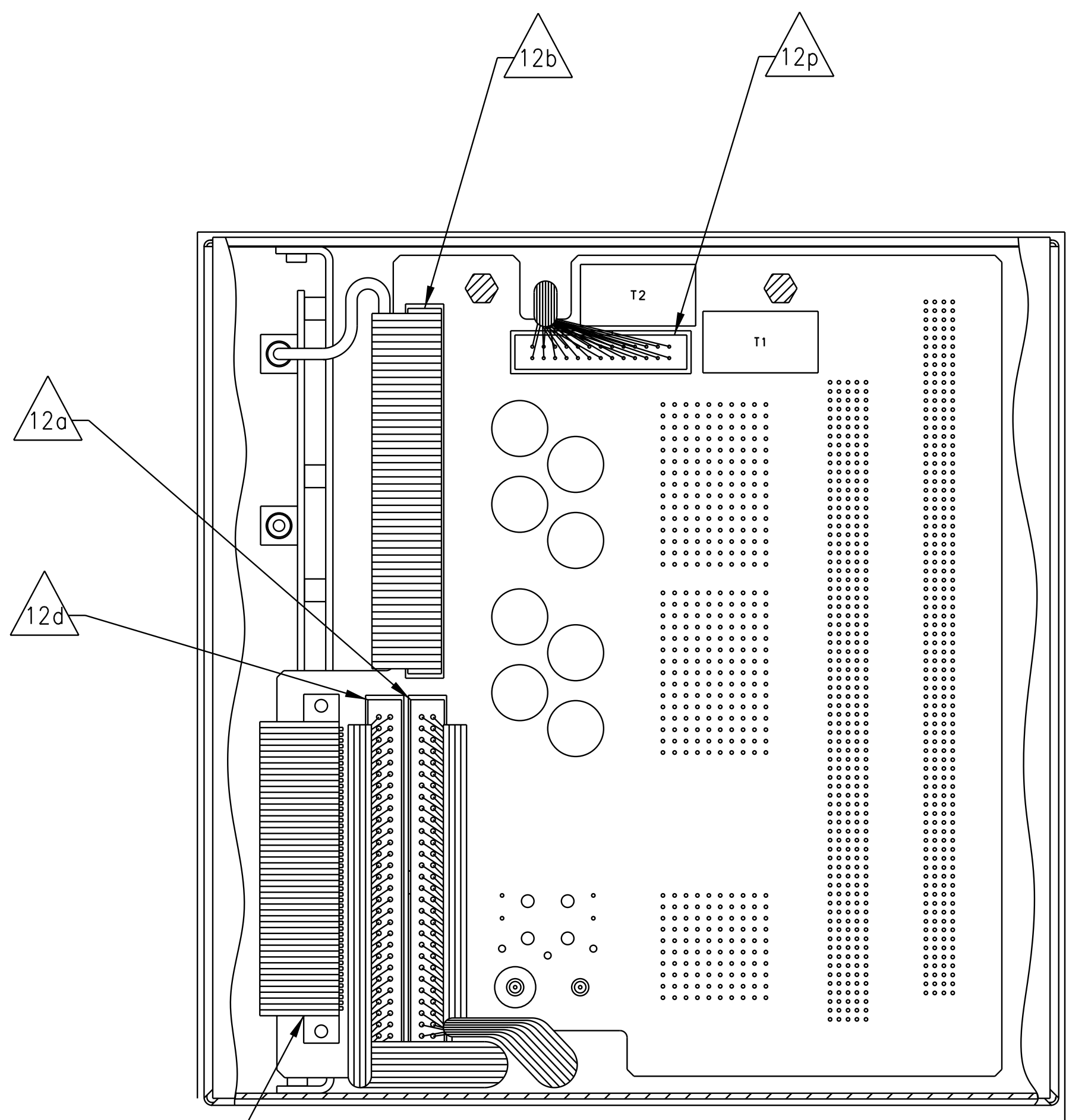
SECTION G-G (FROM SH 2, G4) ARINC CONNECTOR (A1J1) OMITTED FOR CLARITY
