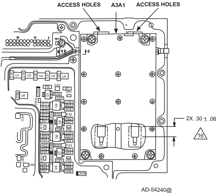
Figure B-2. Transmitter Assembly
