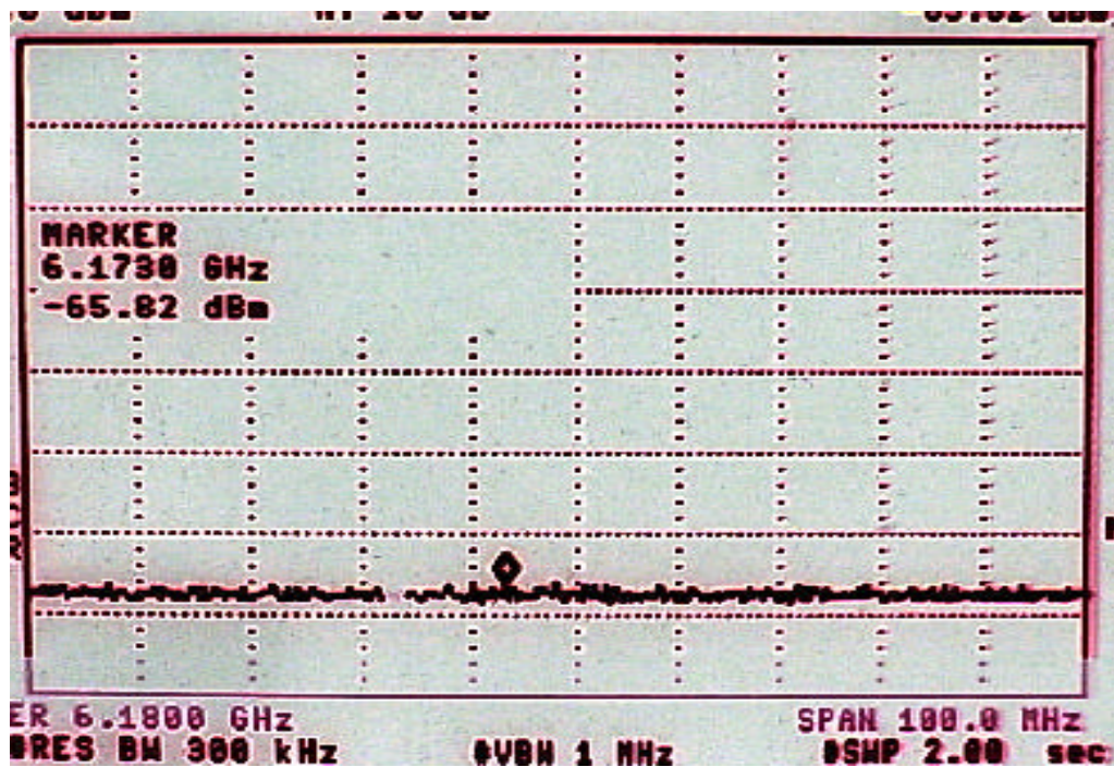
Figure 43: 6 th Harmonic
