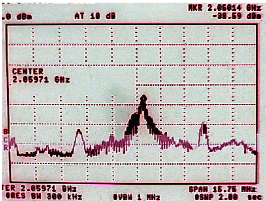
Figure 39: 2 nd Harmonic
