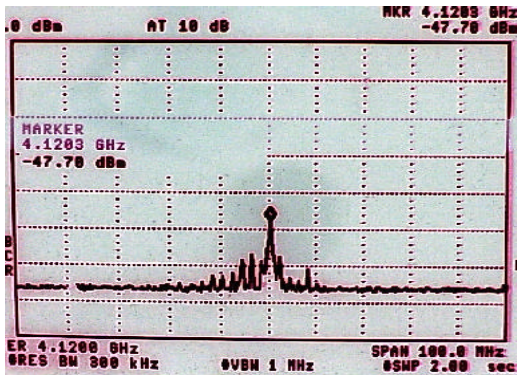
Figure 41: 4 th Harmonic
