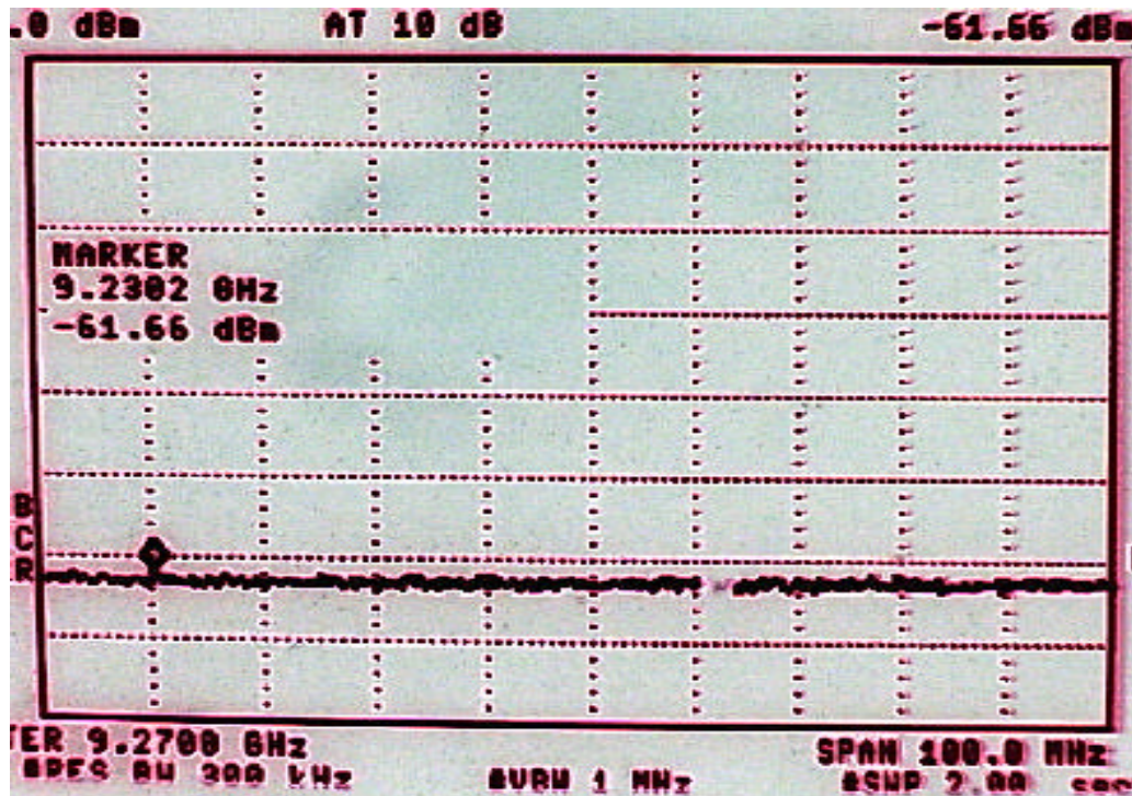
Figure 46: 9 th Harmonic
