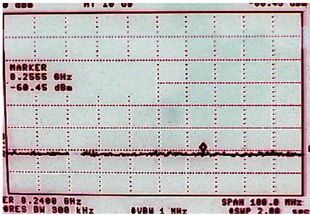
Figure 45: 8 th Harmonic
