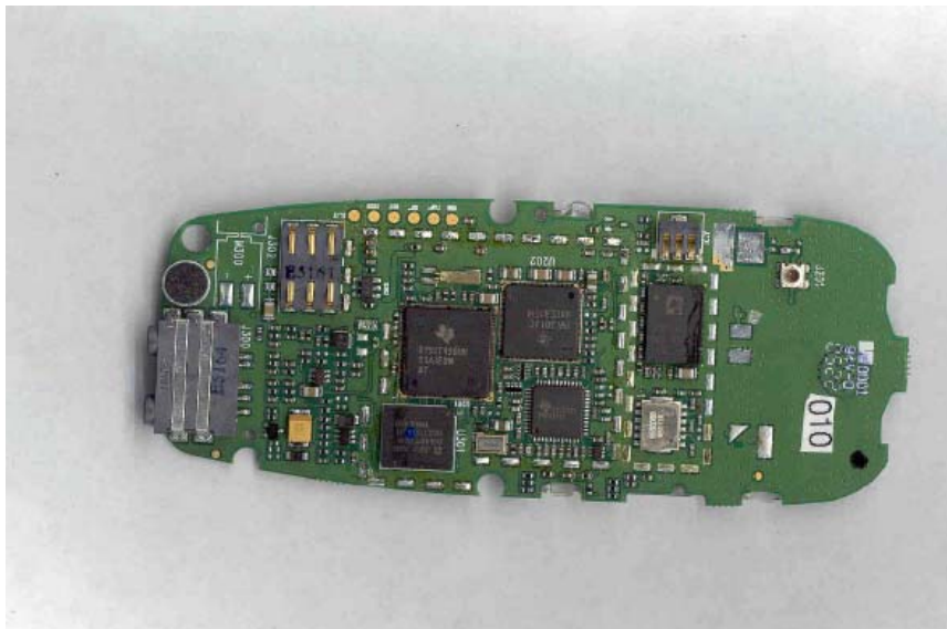
EUT Component without Shielding View
