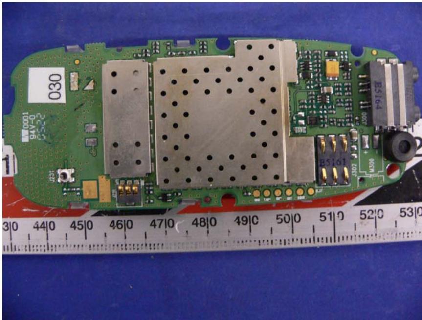
EUT Component with Shielding View
