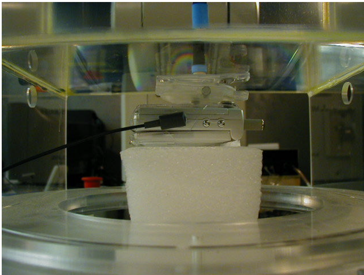
Fig S9. Battery (600 mAH) facing the phantom with Headset.
