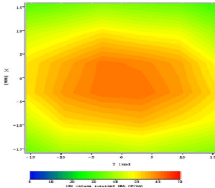
Figure 13. Validation Measurement - 1800 MHz in head tissue
