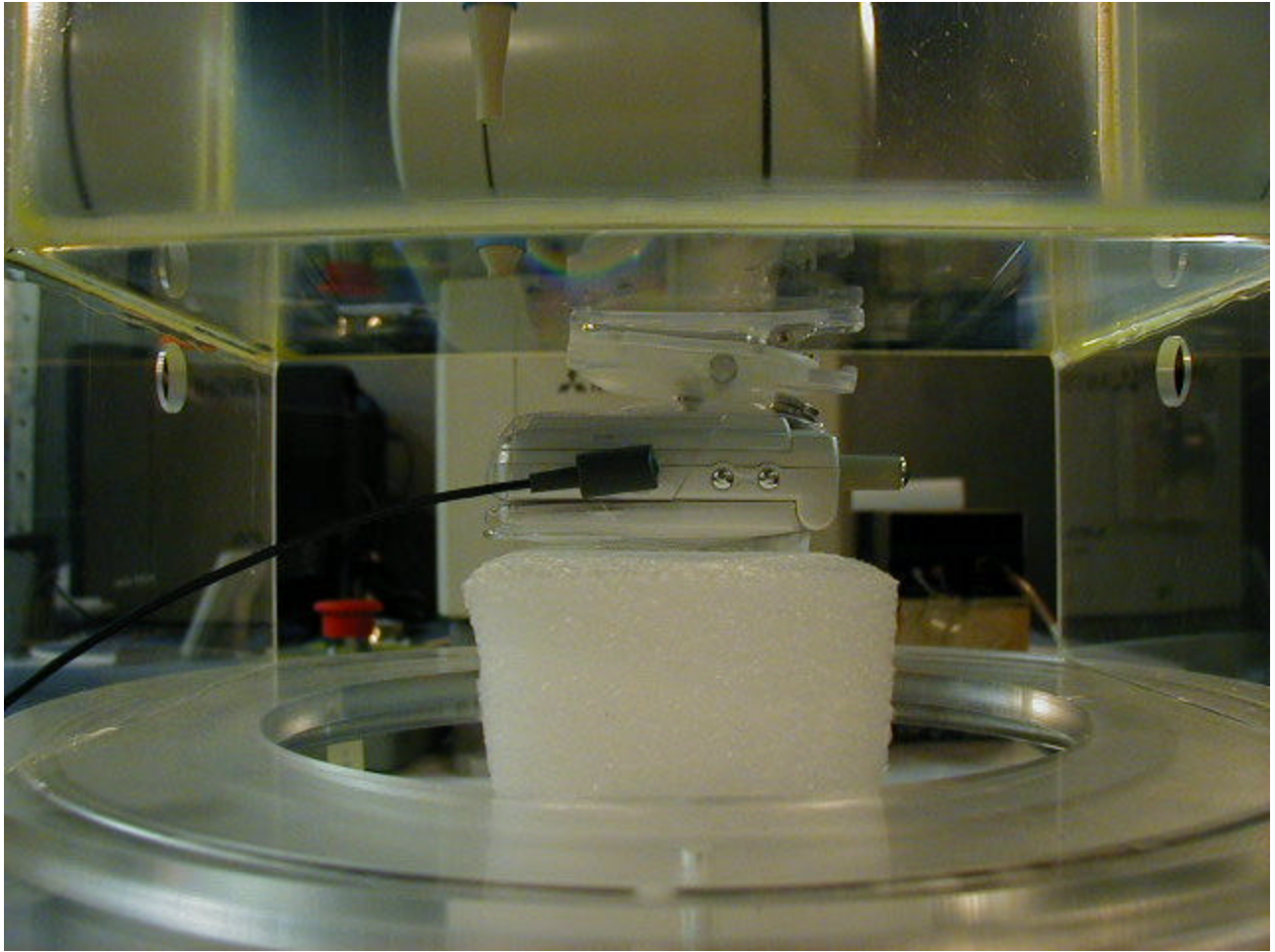
Fig S10. Battery (700 mAH) facing the Phantom with Headset.
