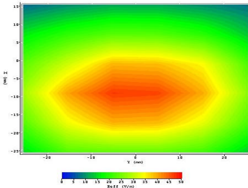
Figure 13. Validation Measurement - 1900 MHz in head tissue
