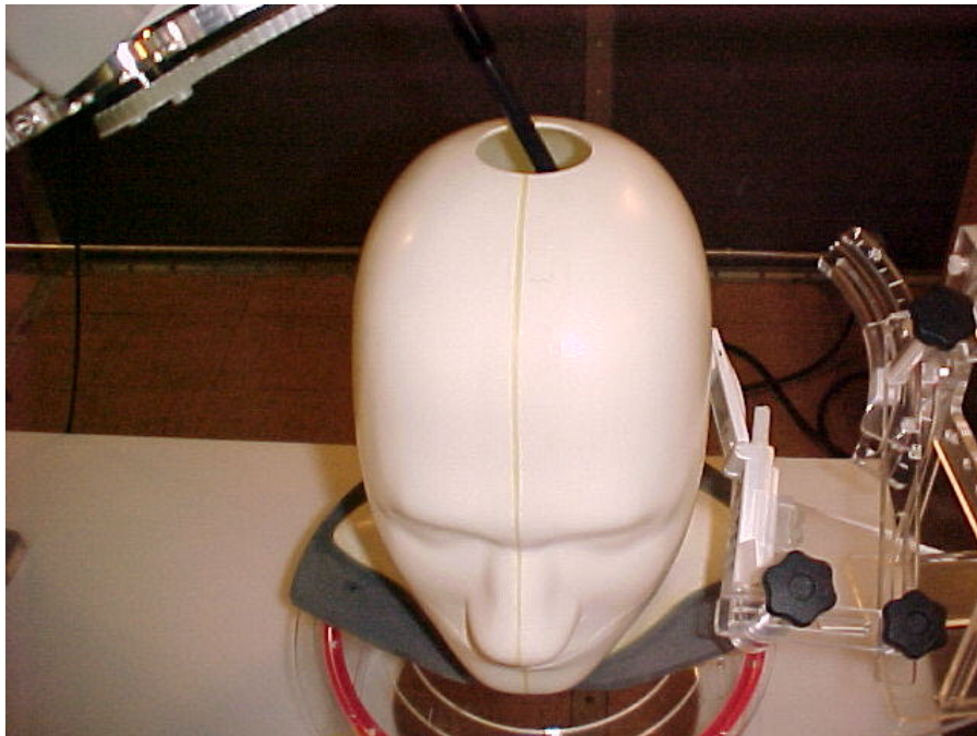
Fig S2. Configuration 2, per table 6
