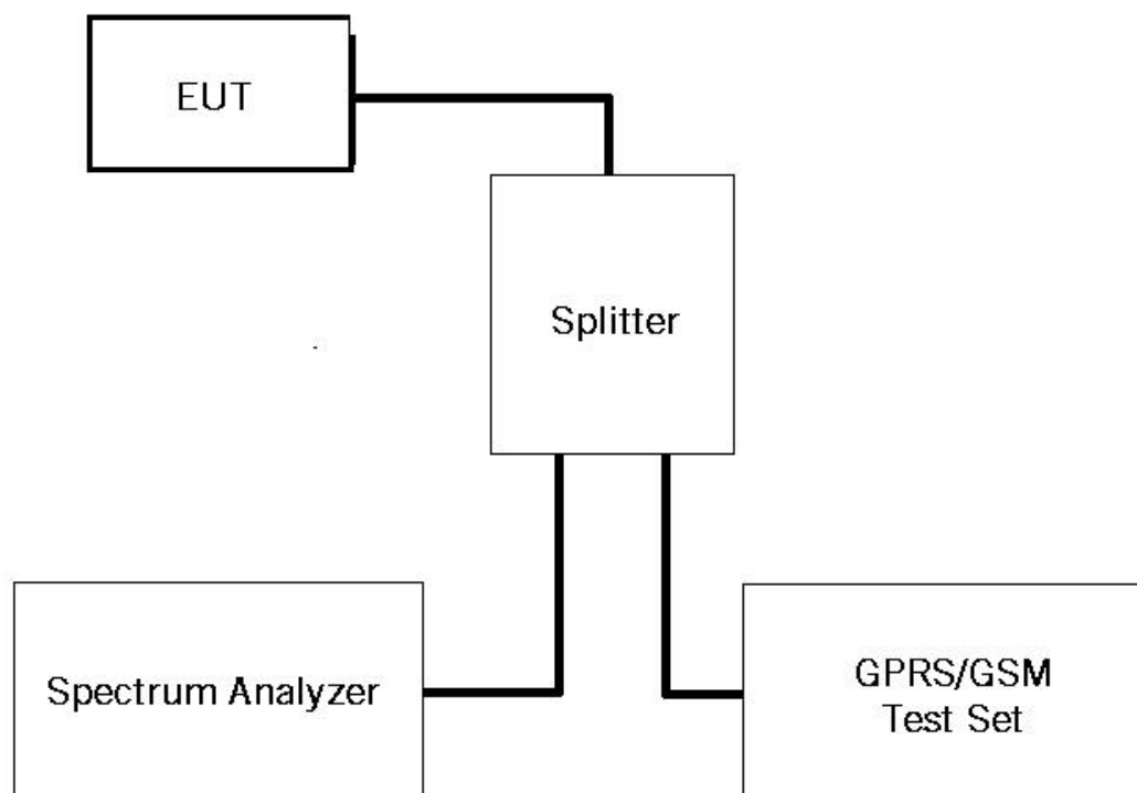
Figure 1 Direct Measurement Configuration
