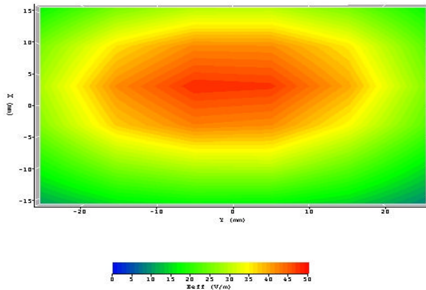
Figure 14. Validation Measurement - 1800 MHz in Head Tissue
