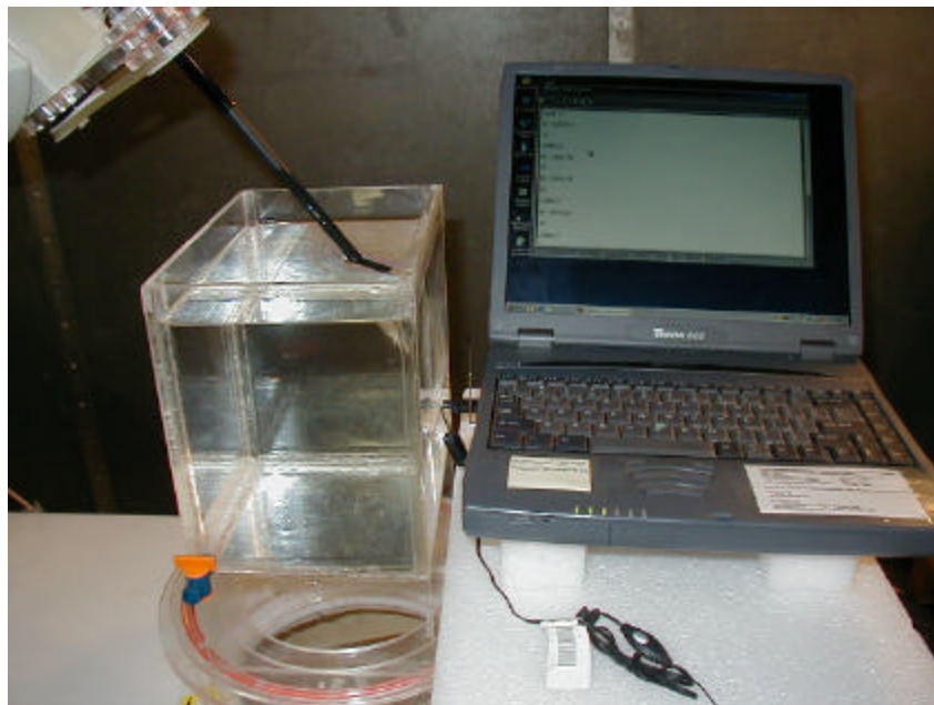
Figure S9. Configuration 2 per Table 10 (Antenna separated from box phantom by 15 mm)
