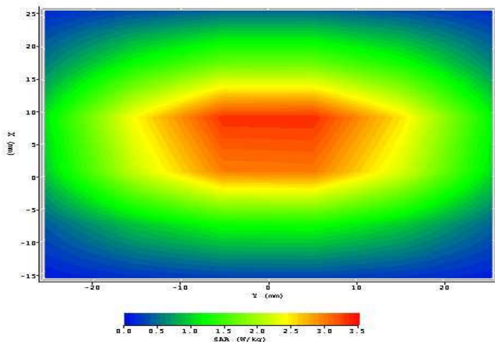
Figure 14. Validation Measurement - 1800 MHz in Head Tissue
