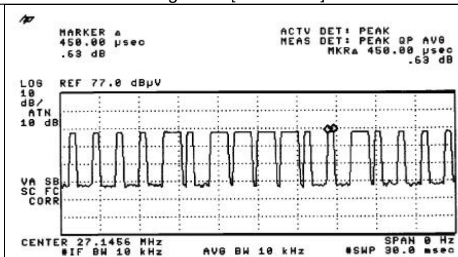
Figure C [Short Pulse]
