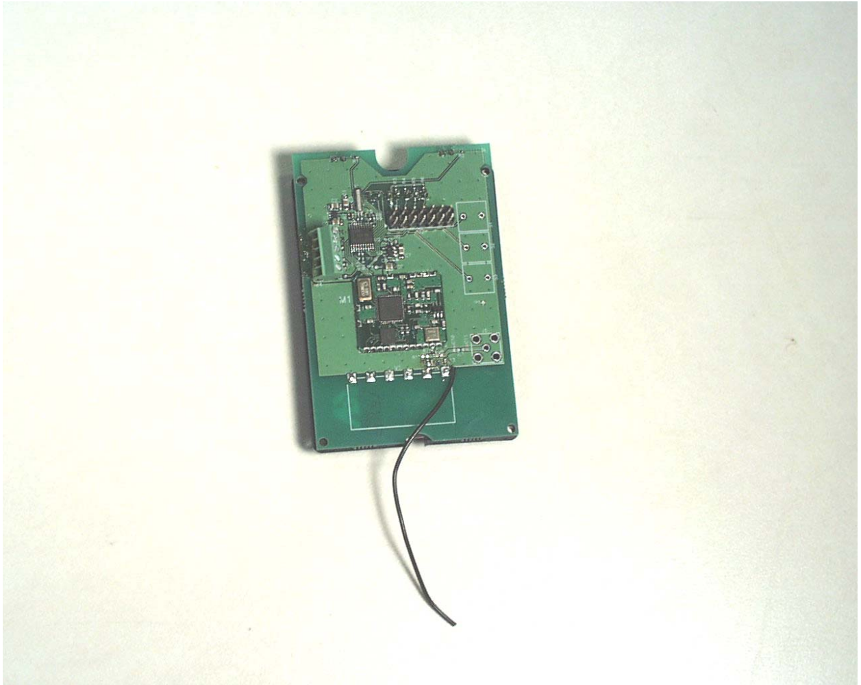
Back View of the 050305 Wireless Numeric Keypad
