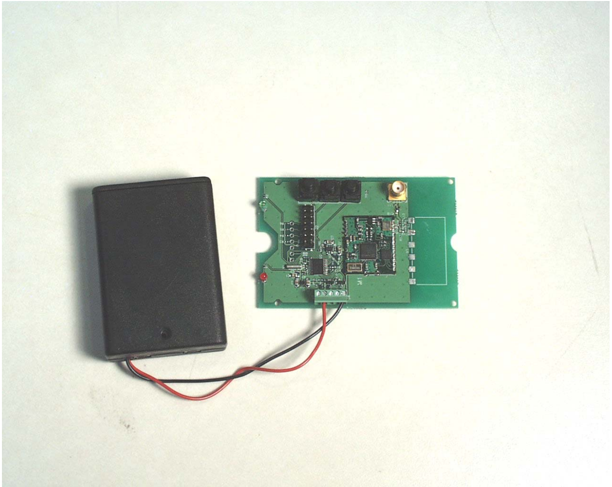
Top View of the 050306 Wireless Numeric Receiver
