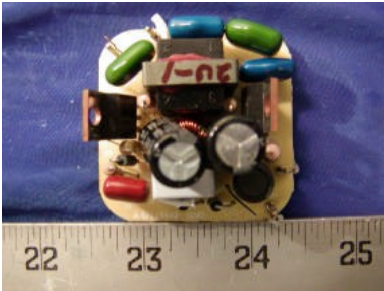
EUT - Component View (RPW-20E)
