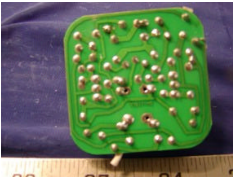
EUT – Solder View (RPW-20E)
