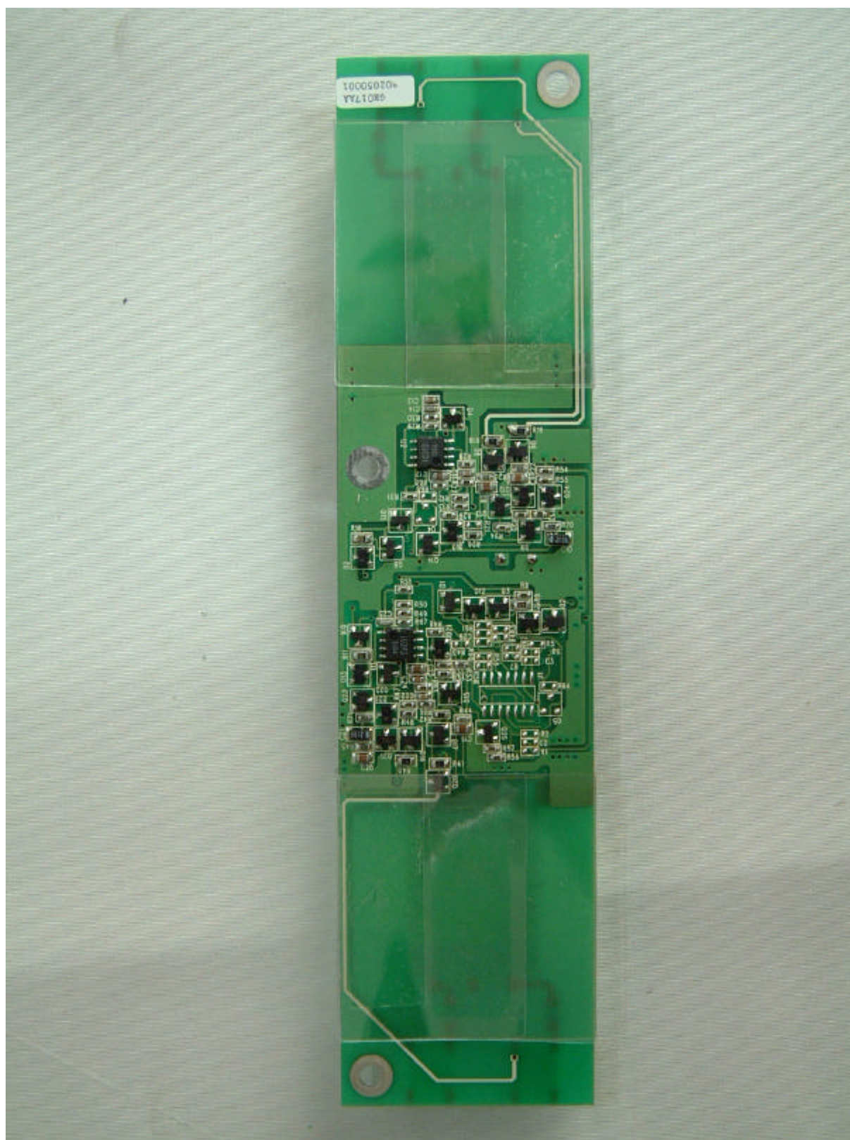
<REAR VIEW OF LCD Board>
