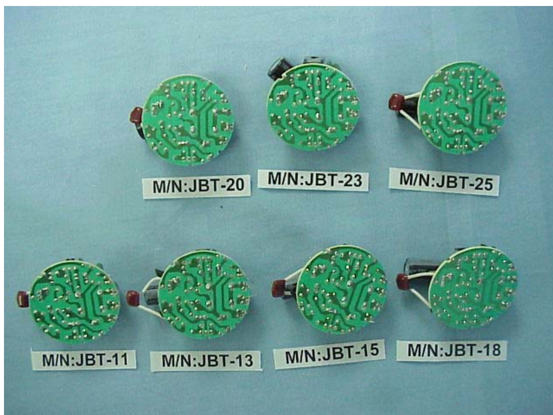
FIGURE 12 ELECTRONIC ENERGY SAVING LAMP (M/N: JBT SERIES) MAIN BOARD (SOLDERED SIDE)
