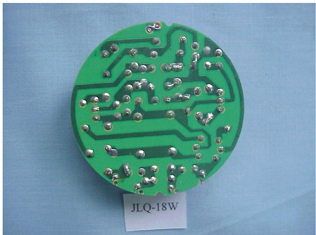
FIGURE 15 ENERGY SAVING LAMP (M/N: JLQ-18W) MAIN BOARD (SOLDERED SIDE)
