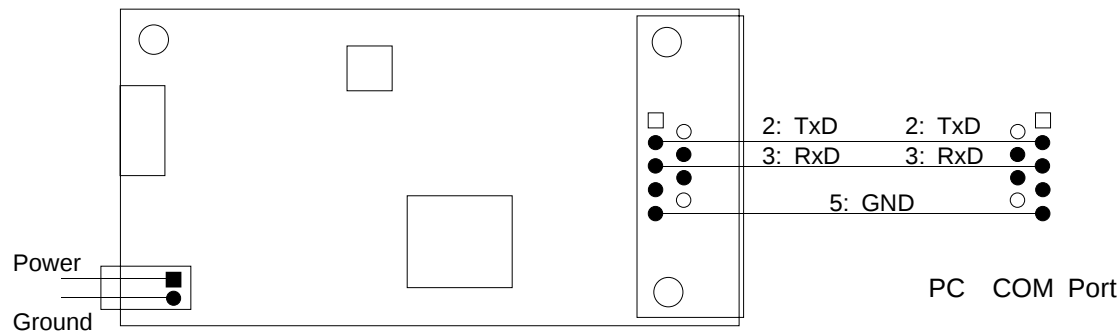
RS-232 Communication Diagram External Power:
