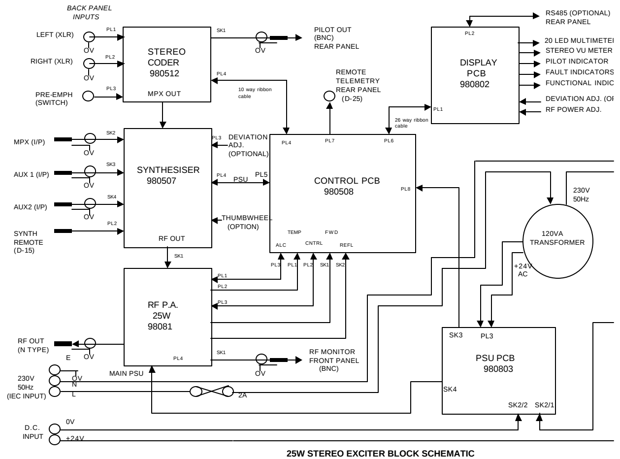
Figure 2: Block diagram of FM-25
