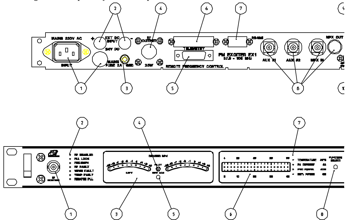
Figure 1: Front panel layout and rear panel connectors and functions
