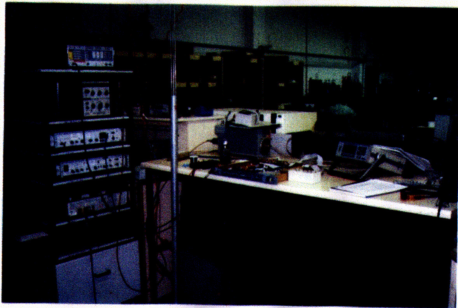
Bench test setup for testing of FM-25 25W Stereo Transmitter showing connection to equipment test rack
