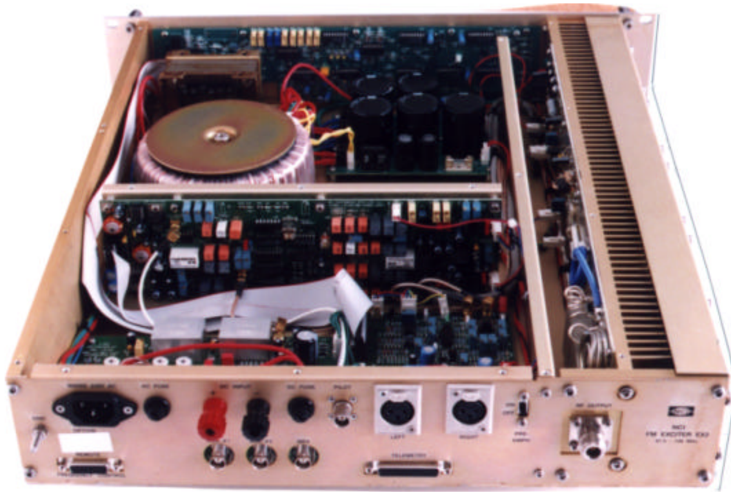
Internal view of the FM-250 250W Stereo Transmitter
