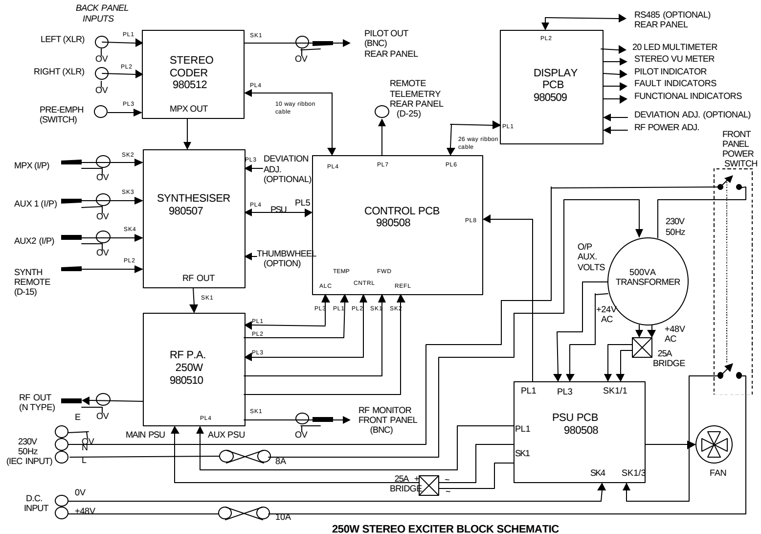
Figure 3: Block diagram of FM-250
