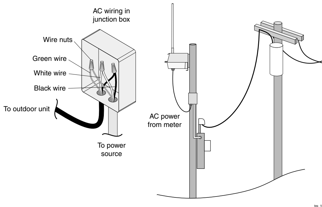
Figure 16 Connecting Category C AC Power
