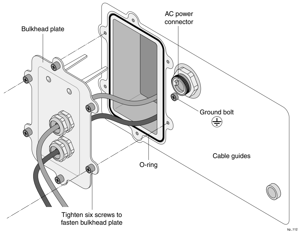
Figure 21 Data Port Connection
