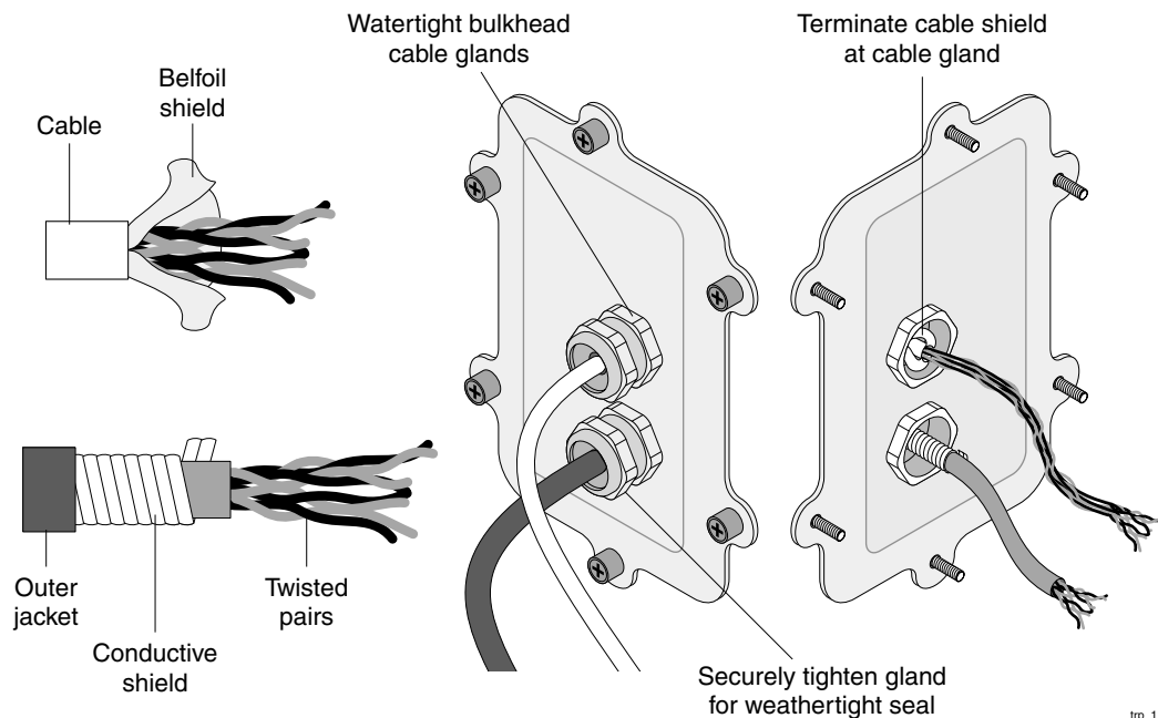
Figure 20 Data Cable Detail
