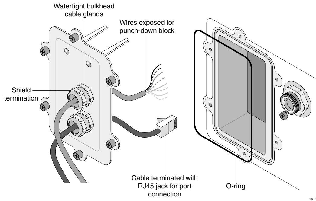
Figure 19 Options for Connecting a Data Port
