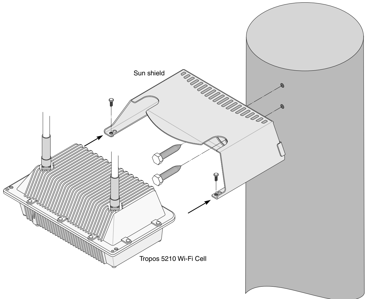
Figure 7 Wood Pole Mounting
