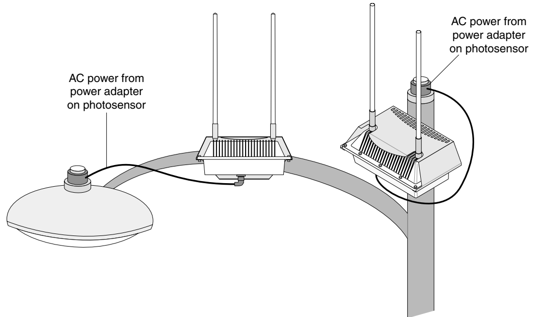
Figure 18 Connecting Streetlight Power
