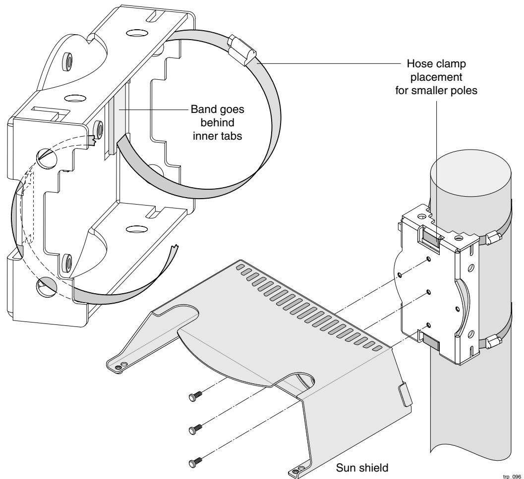
Figure 4 Proper Use of Hose Clamps - Small Poles (< 8 Inches)
