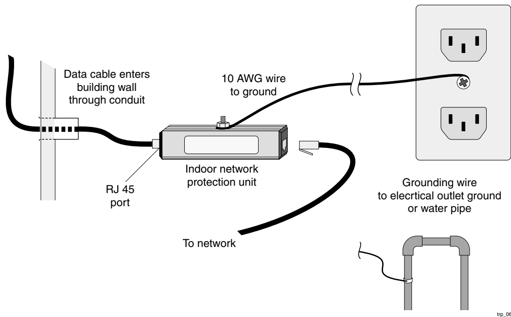
Figure 14 Grounding the Indoor Network Protection Unit
