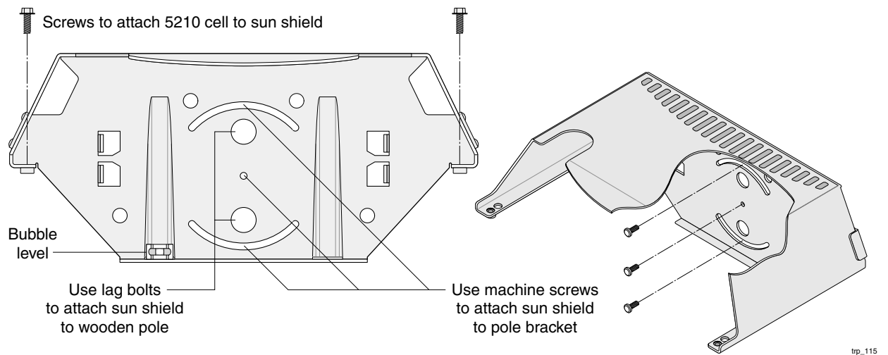
Figure 6 Sun Shield Connections
