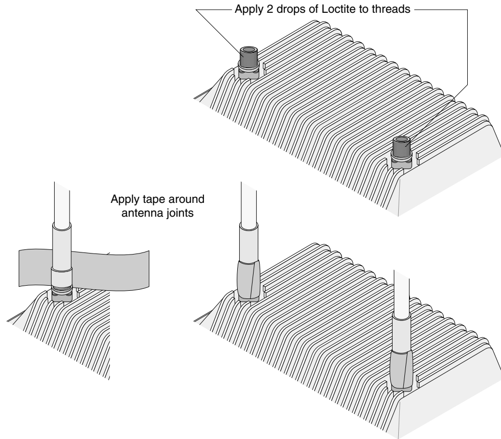
Figure 11 Waterproofing Antenna Connections
