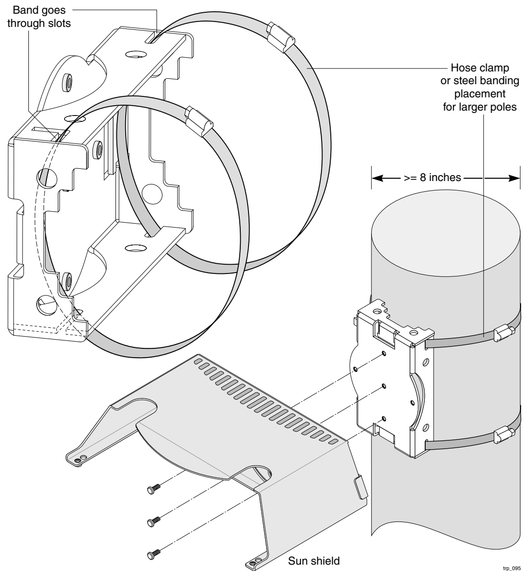
Figure 3 Proper Use of Hose Clamps - Large Poles ( \geq 8 Inches)
