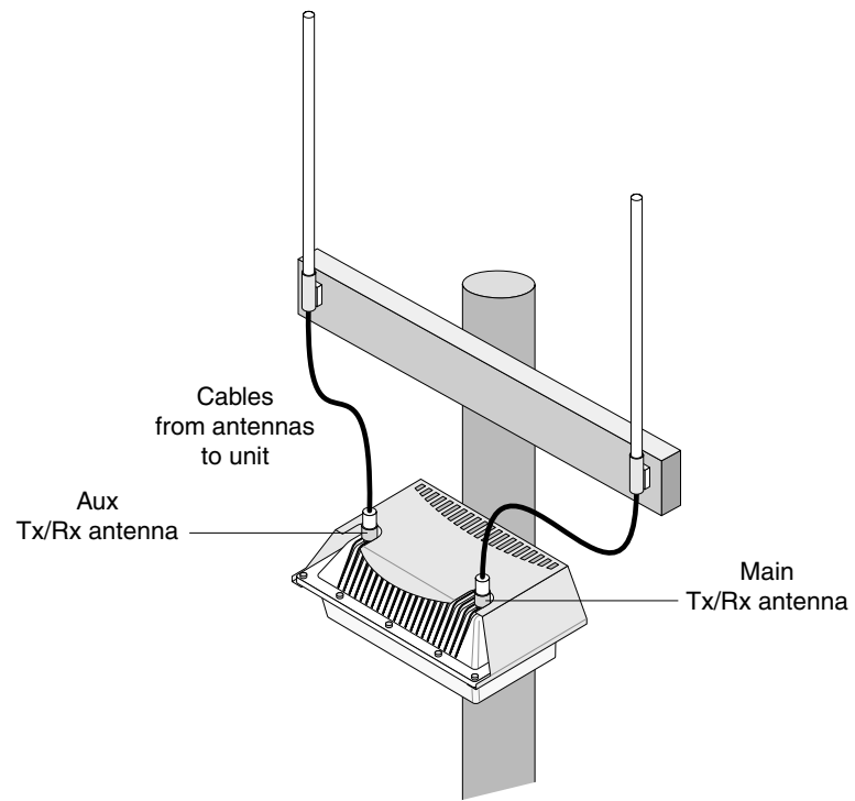
Figure 10 Connecting External Antennas
