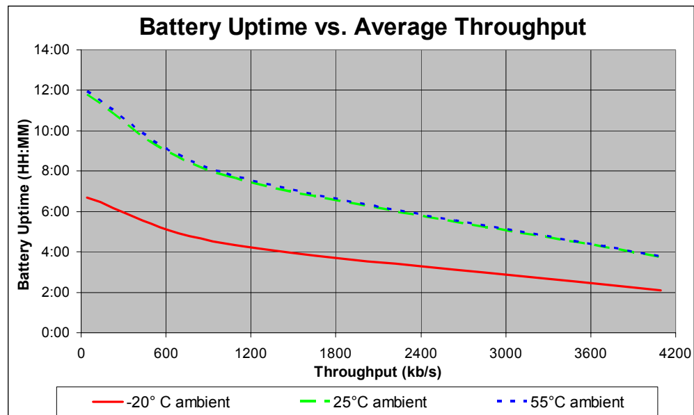
Figure 24 Average Battery Backup Time
