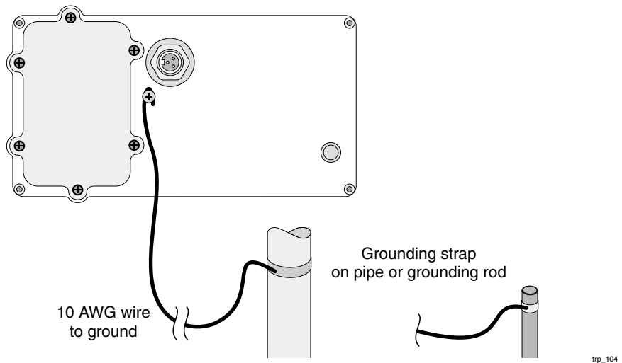
Figure 13 Ground Arrangement
