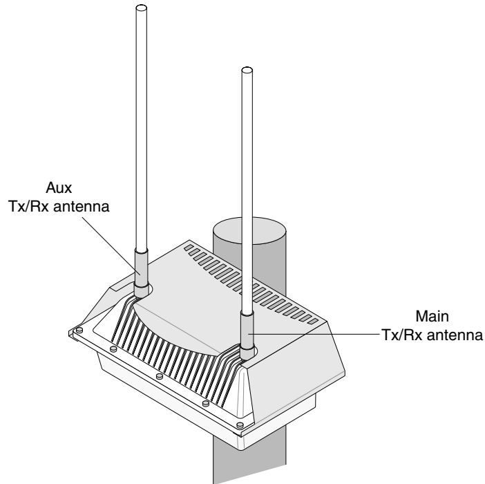
Figure 12 Replacing Tropos 5210 Wi-Fi cell Antennas
