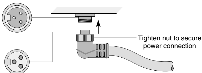
Figure 17 Connecting the AC Power Cable to the Cell
