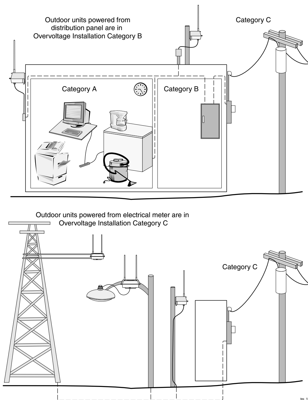
Figure 15 IEEE/ANSI C62.41 Power Categories
