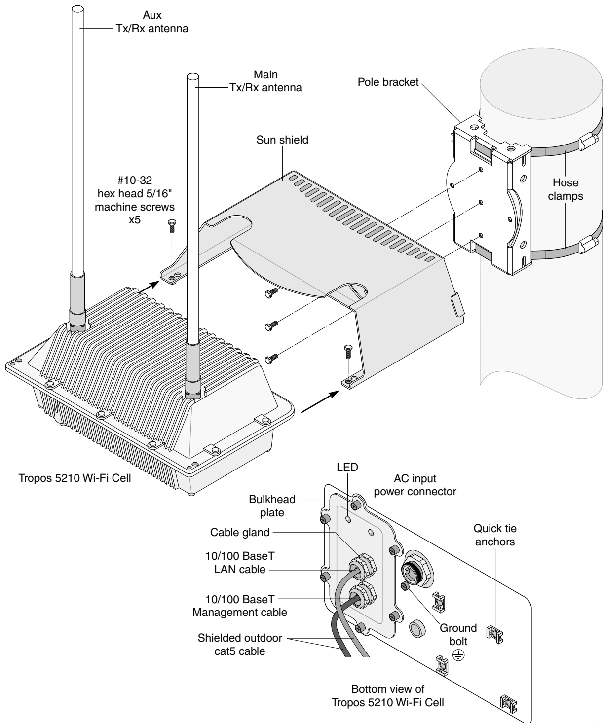
Figure 1 Tropos 5210 Wi-Fi Cell Exploded View
