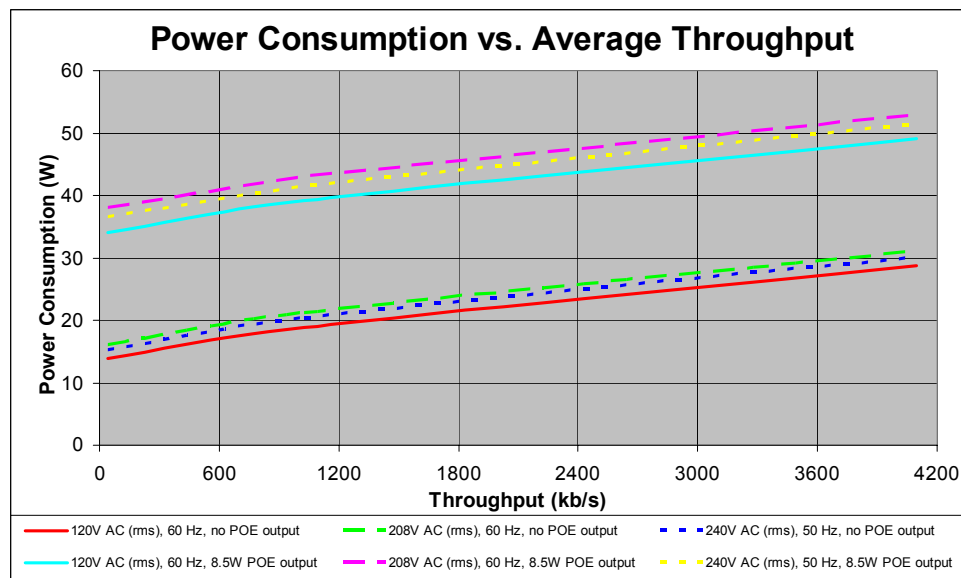
Figure 25 AC Power Consumption
