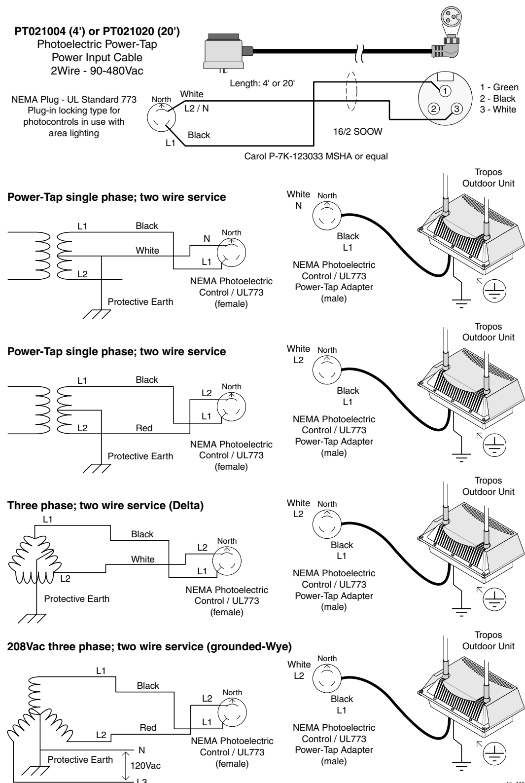
Figure 26 AC Wiring — Photoelectric Power Tap
