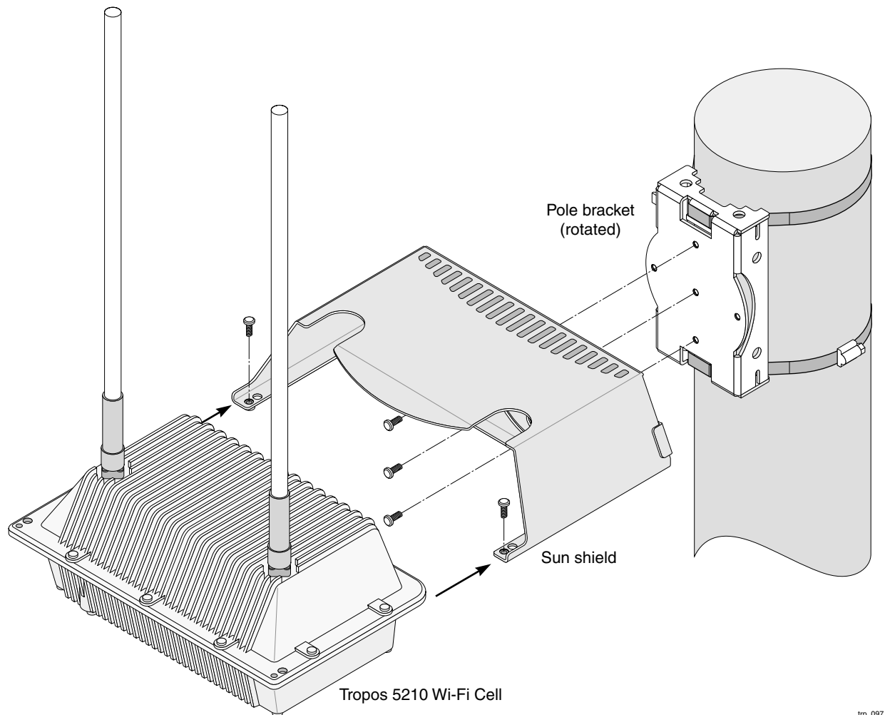
Figure 5 Metal Pole Mounting
