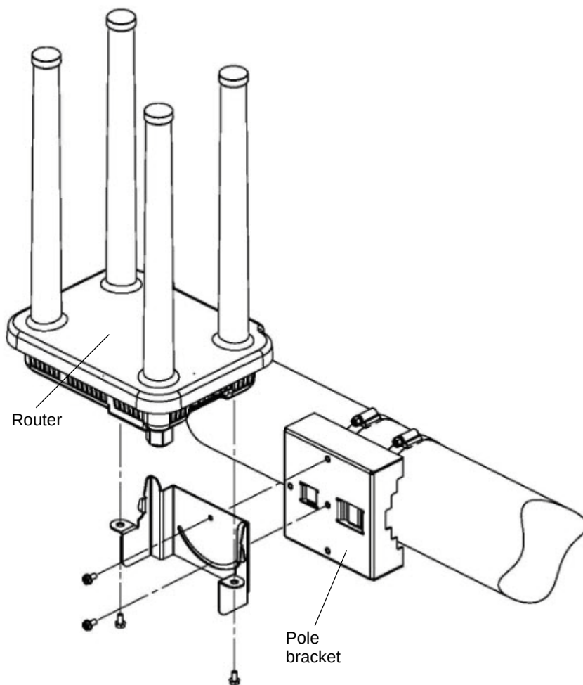
FIGURE 9 Streetlight Mounting
