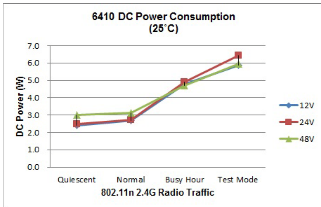
FIGURE 21 6410 Power Consumption
