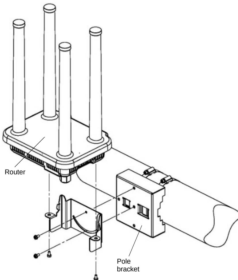
FIGURE 9 Streetlight Mounting
