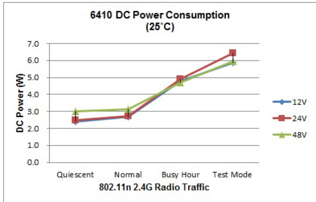
FIGURE 21 6410 Power Consumption
