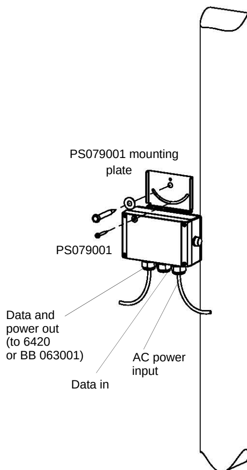
FIGURE 17 Mounting the PS079001 on a Wood Pole
