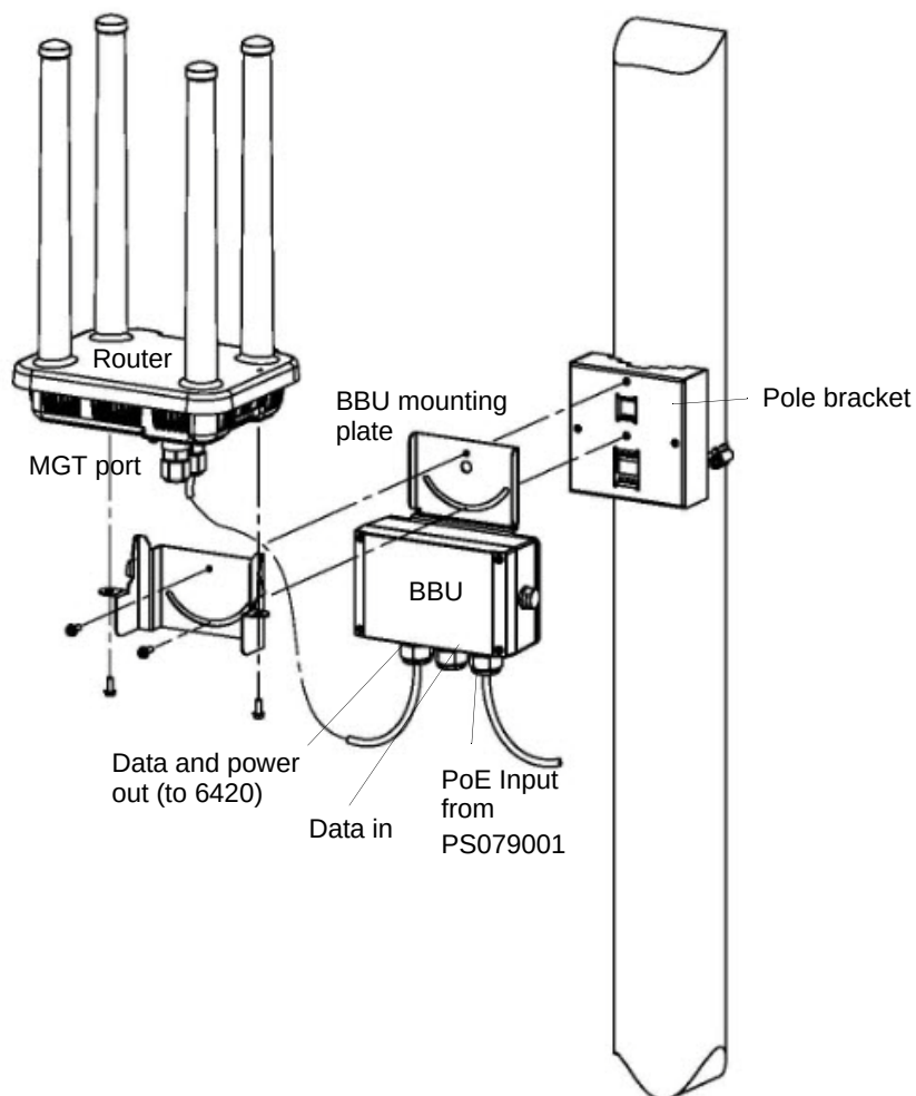
FIGURE 18 Co-Mounting the BBU with the Router
