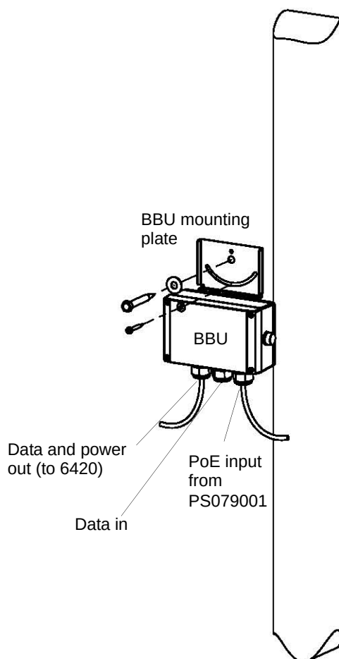
FIGURE 20 Mounting the BBU on a Wood Pole
