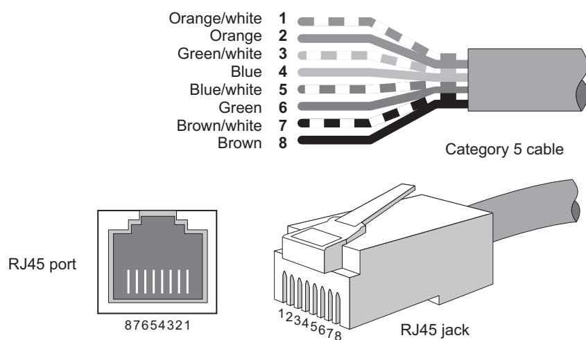
Figure 33 Cable Preparation and Termination
