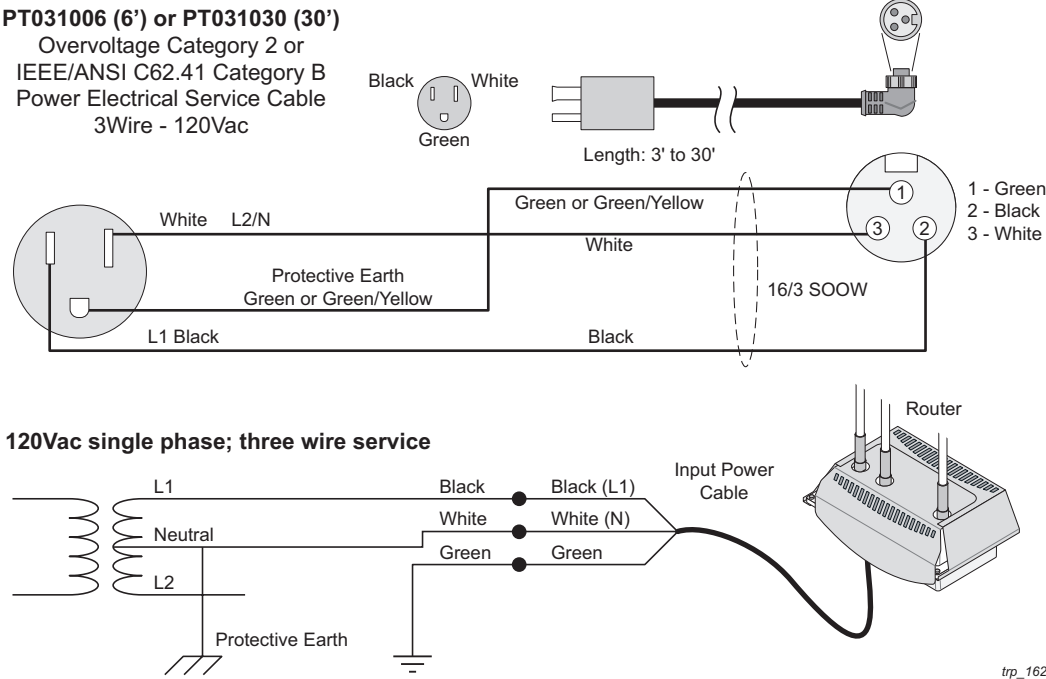
Figure 28 AC Wiring Power Cable 120VAC, 15A Plug
