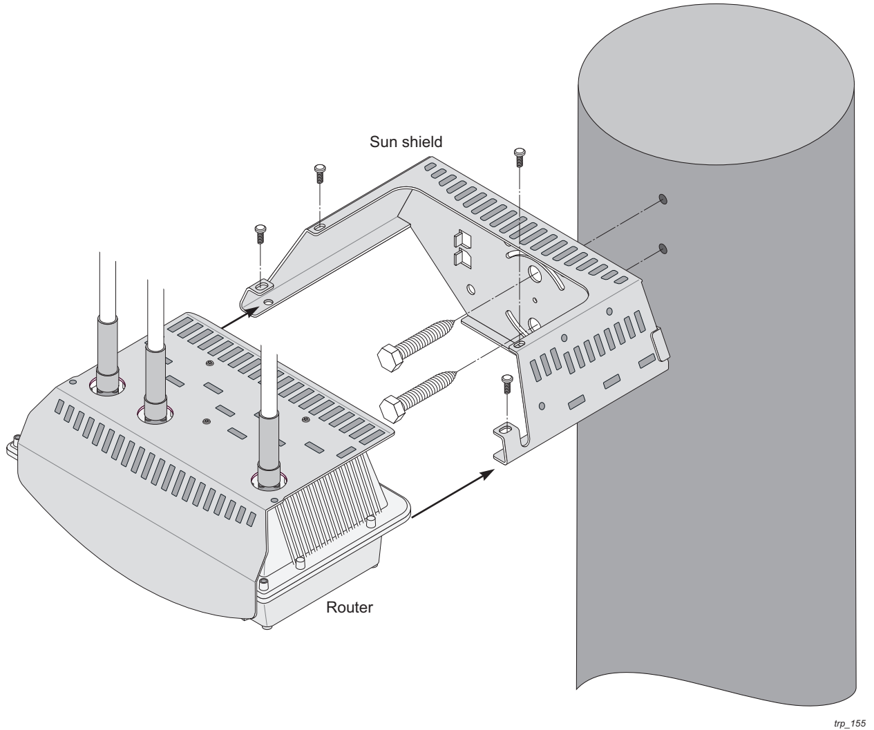
Figure 6 Wood Pole Mounting
