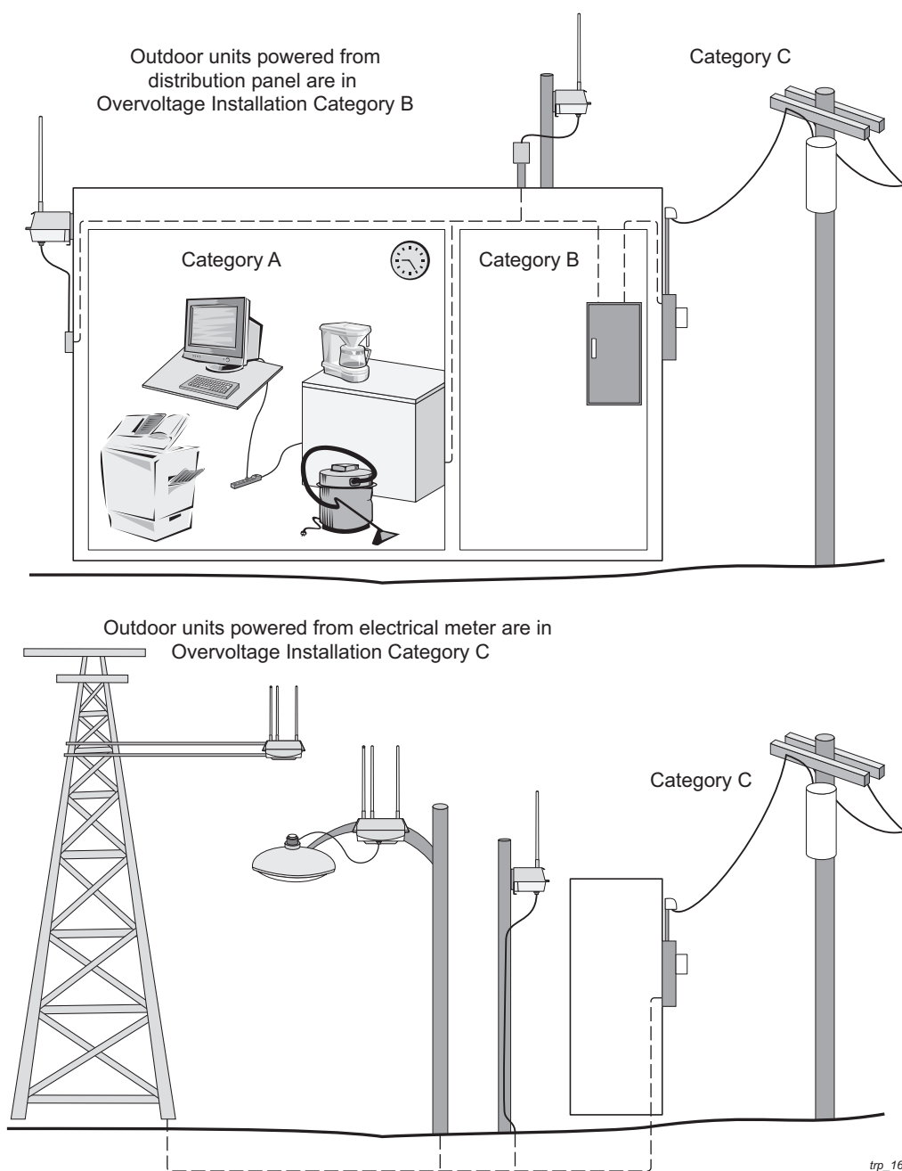
Figure 14 IEEE/ANSI C62.41 Power Categories
