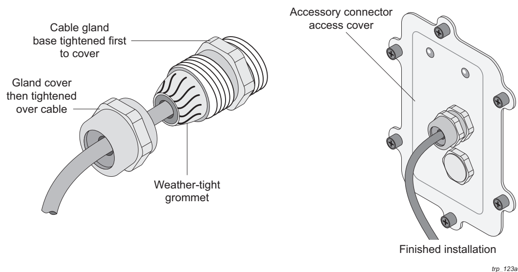
Figure 32 Cable Gland Assembly
