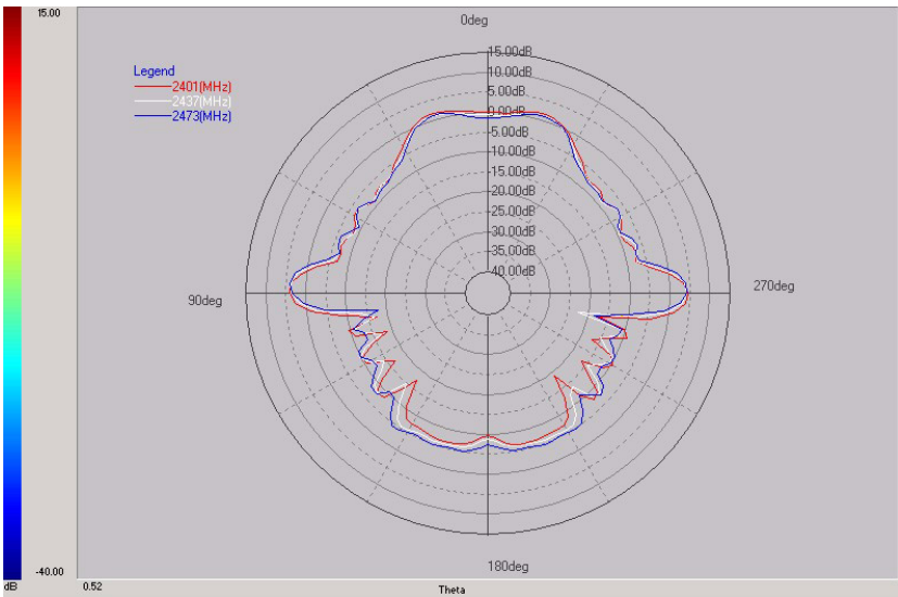
Elevation (Phi=90°)
