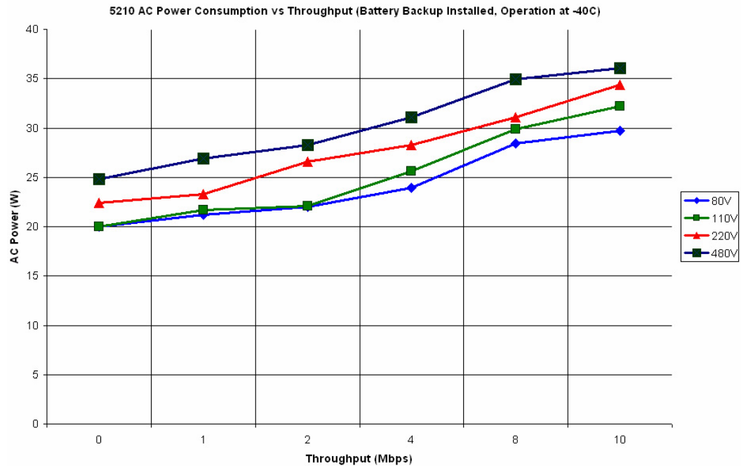
Figure 26 AC Power Consumption vs. Throughput (Battery Backup, -40o C)
