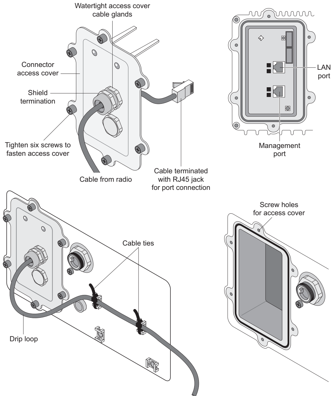
Figure 30 Cable Connections
