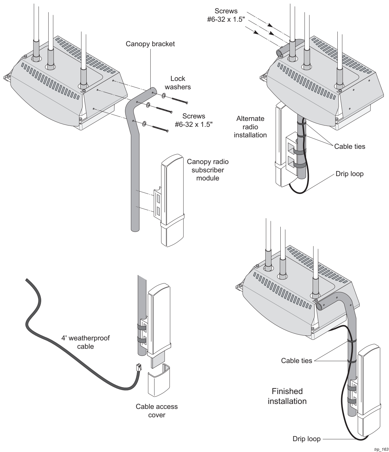
Figure 29 Canopy Assembly
