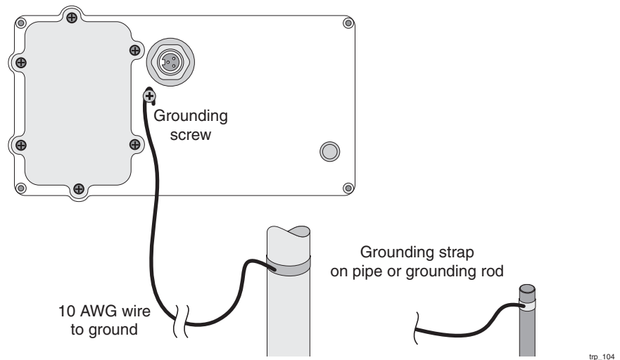
Figure 12 Grounding Arrangement
