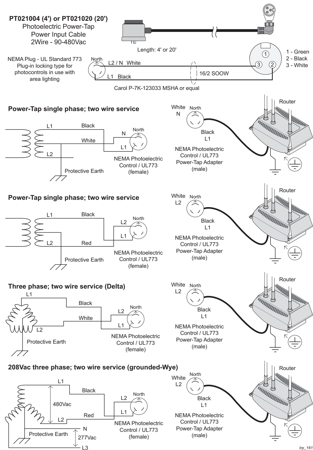
Figure 27 AC Wiring — Photoelectric Power Tap
