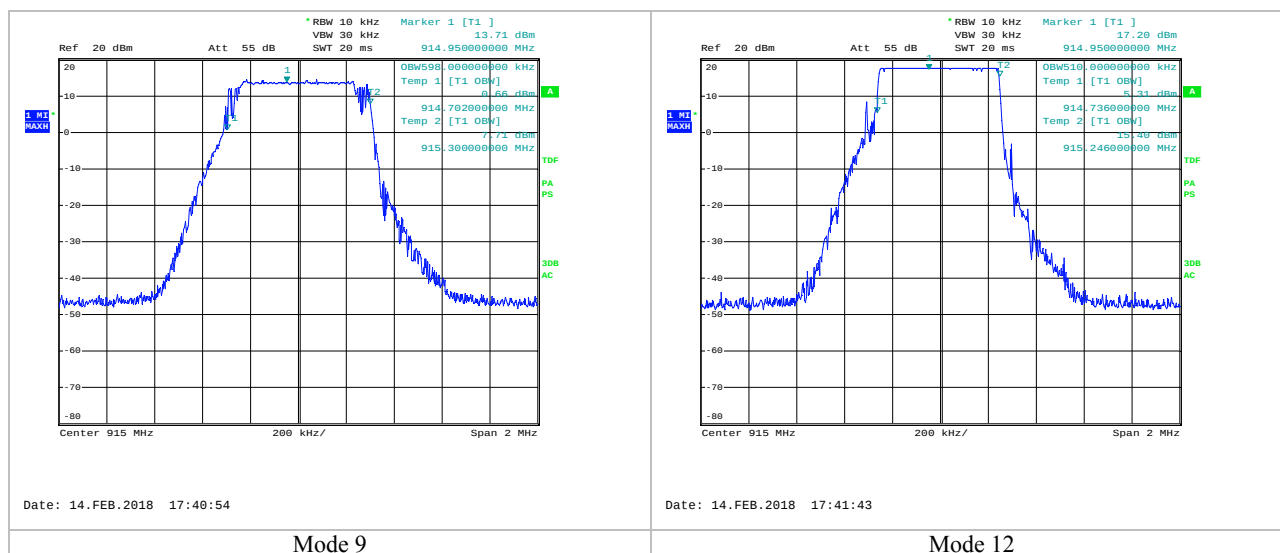
Occupied Bandwidth
