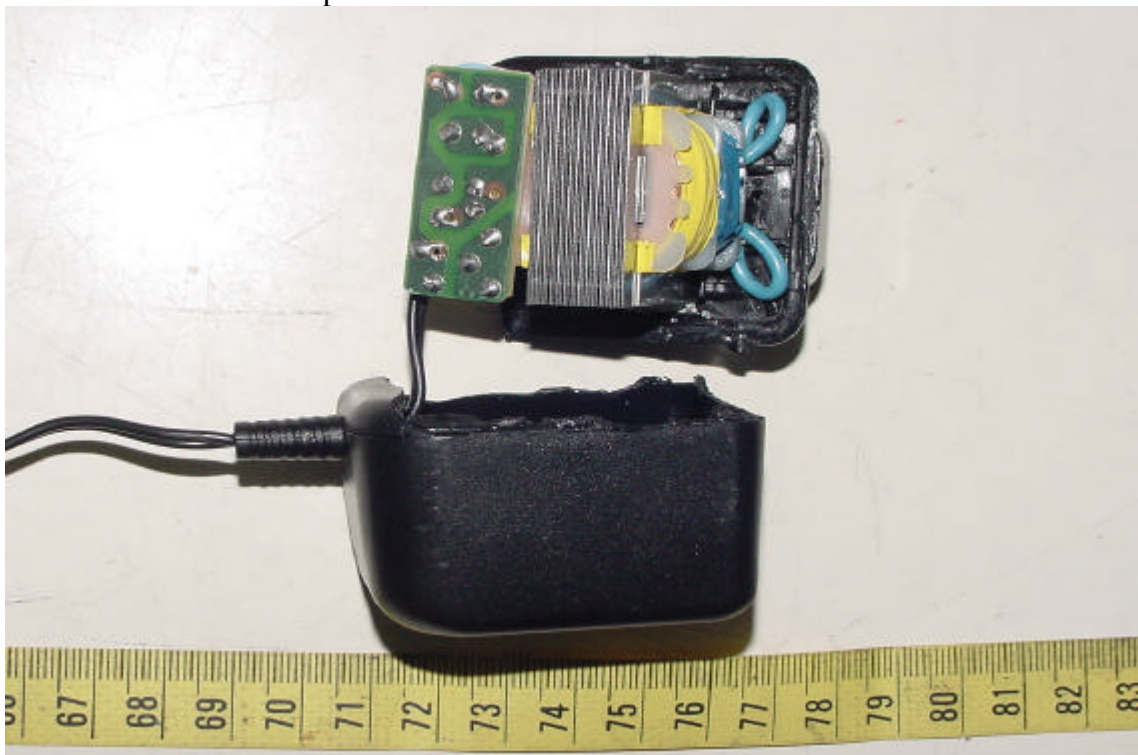
18. Internal View of Adaptor PCB
