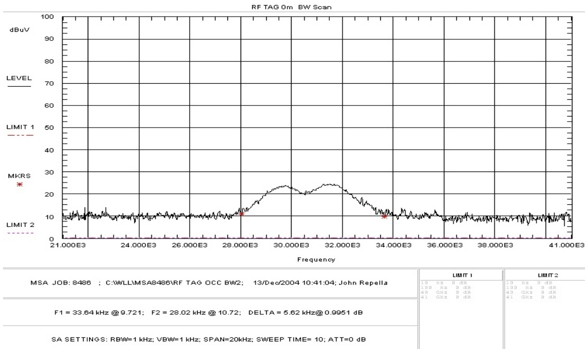
Figure 1. Occupied Bandwidth
