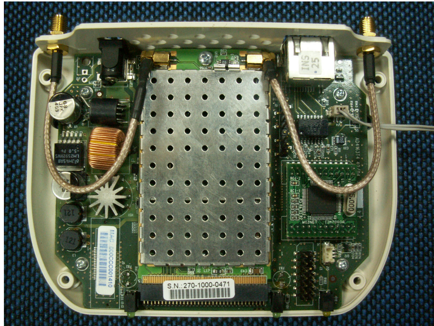
Figure 5 PCB in Case
