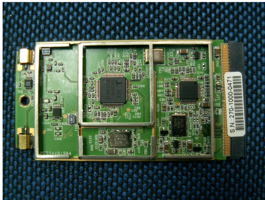
Figure 9 PCB 2 Side 1 Without Shield
