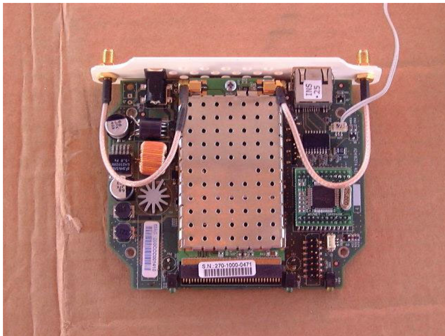
Figure 6 PCB 1 + PCB 2
