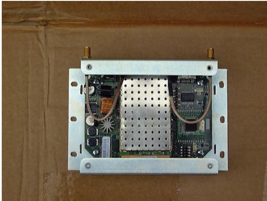
Figure 15 PCB in Case
