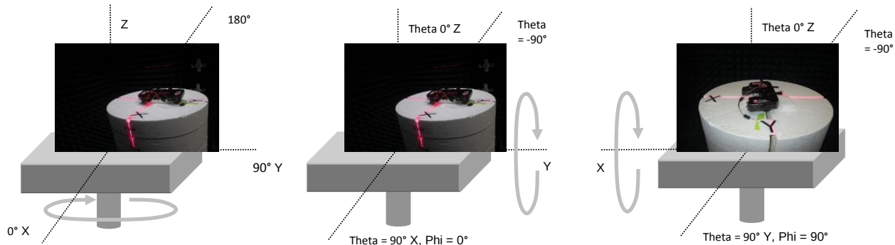
Azimuth Cut (Theta Axis = 90°)
