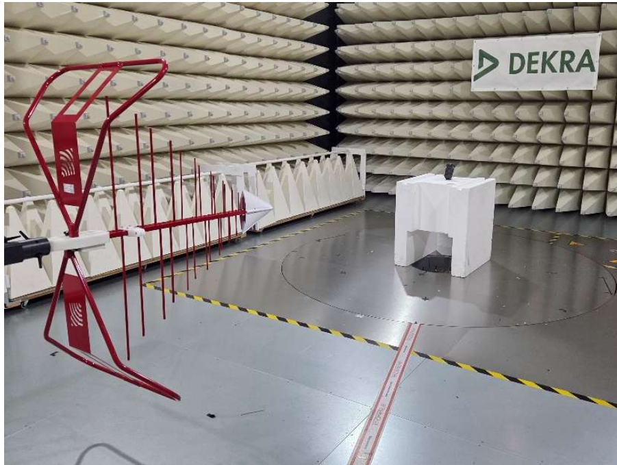
5. Radiated Emission Test Setup 30MHz – 1GHz
