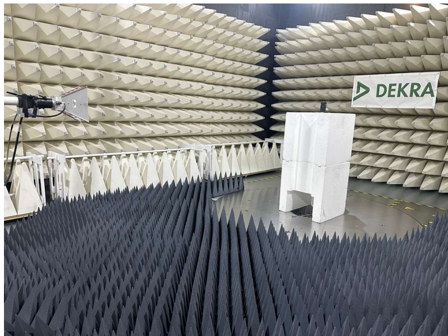
6. Radiated Emission Test Setup 1GHz – 18GHz
