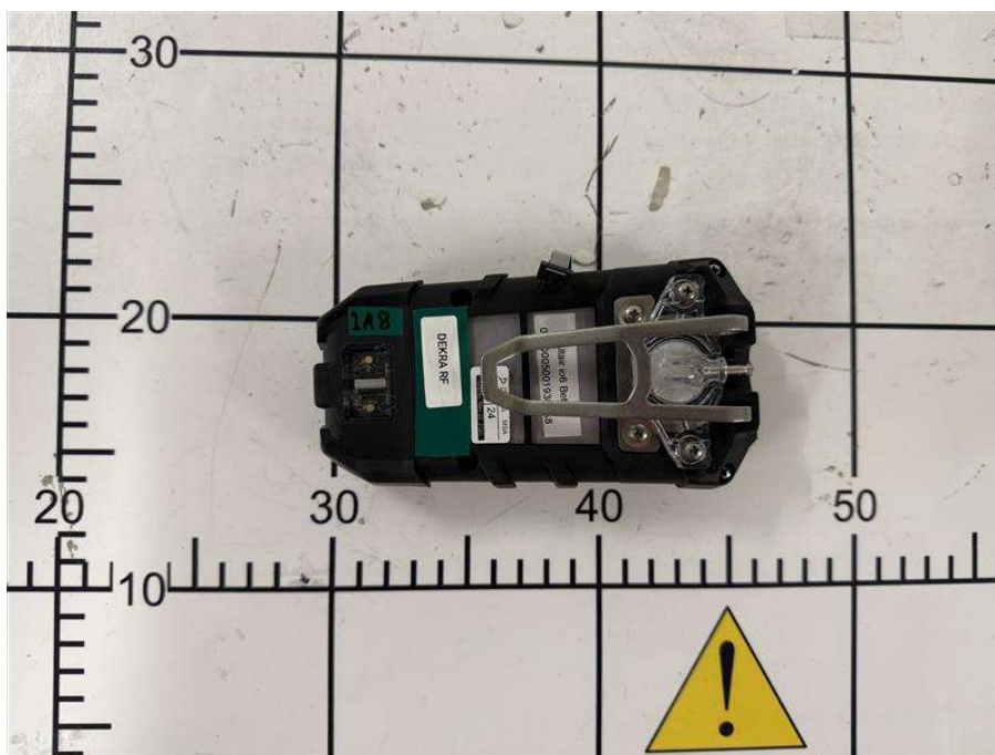
2. Bottom View of the DUT
