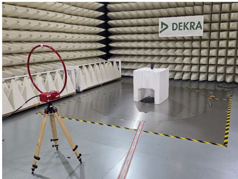
4. Radiated Emission Test Setup 9kHz – 30MHz
