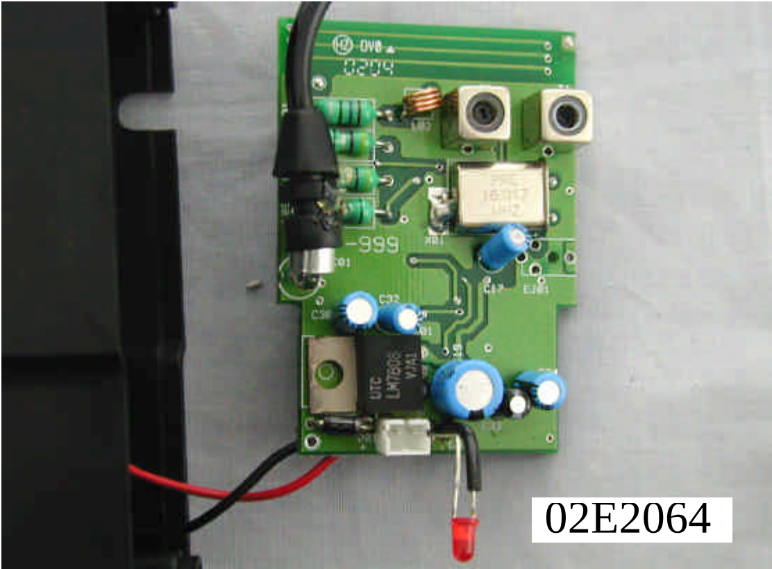
Photo # 3 Unit Partially Disassembled
