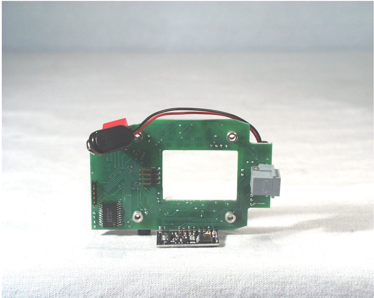
Bottom View of the Main PCB
