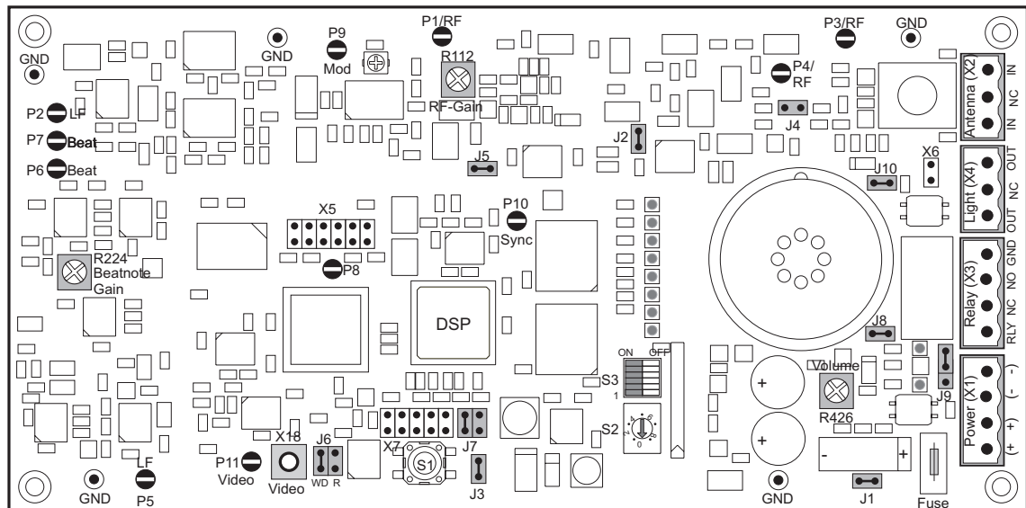
RX Default Jumper Settings Layout
