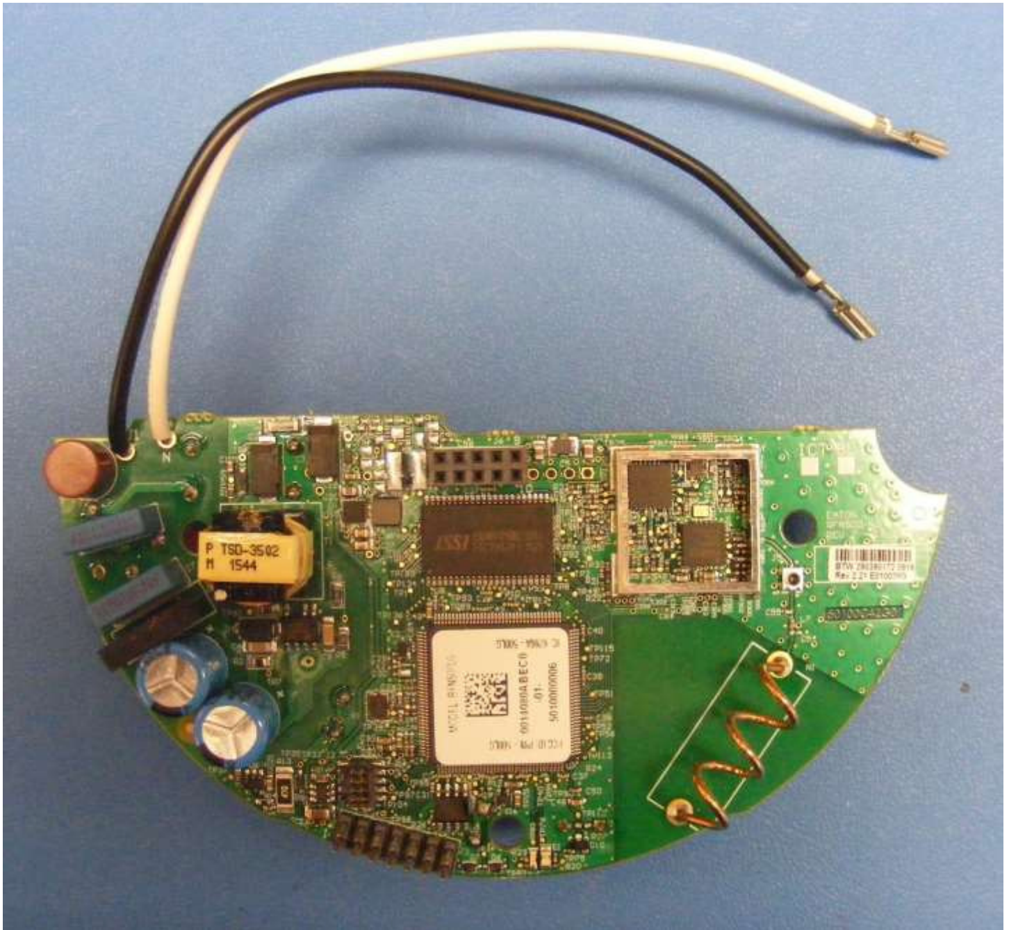
Figure 3: RFN-500LG – Top, shield removed
