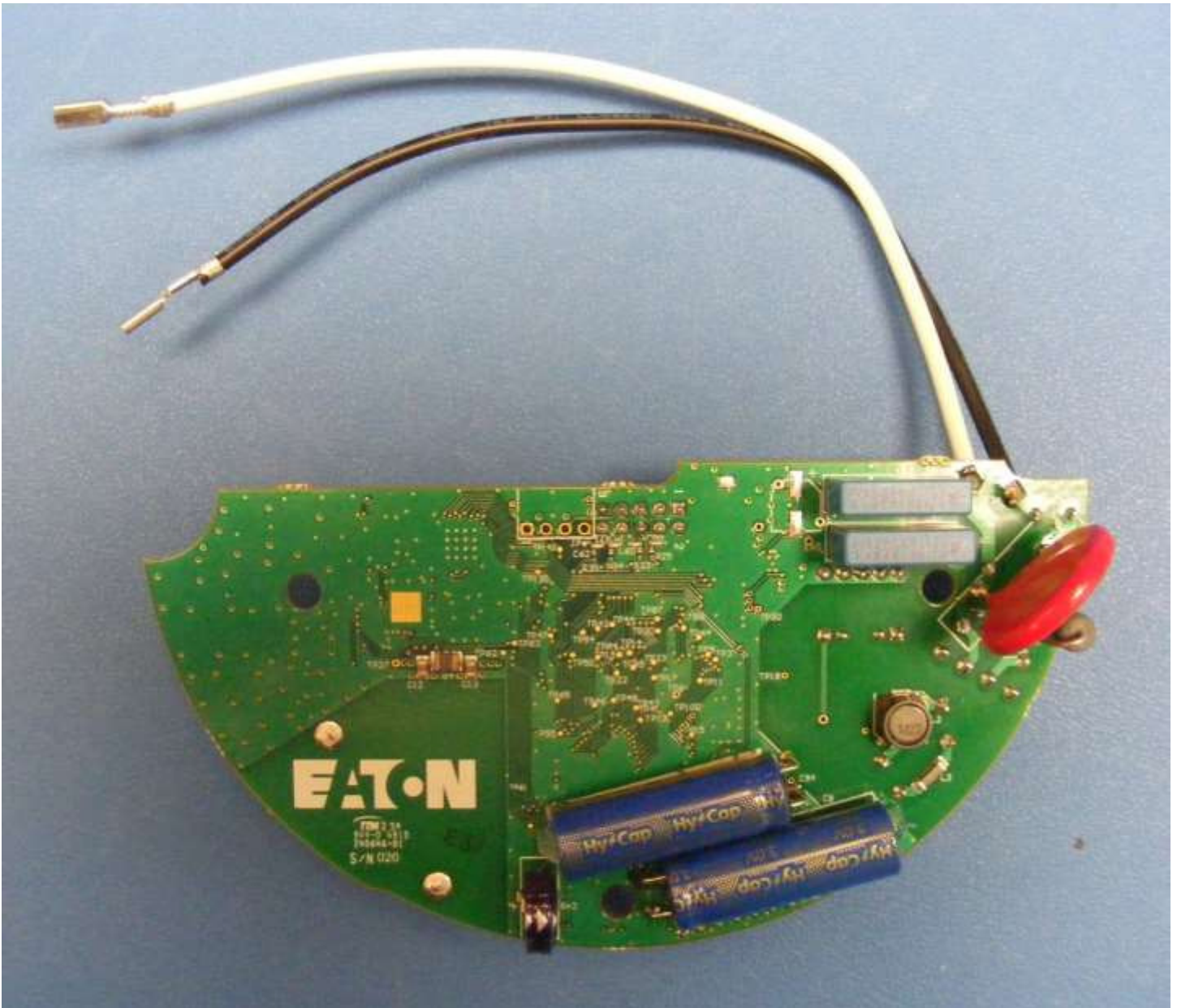
Figure 2: RFN-500LG – Bottom
