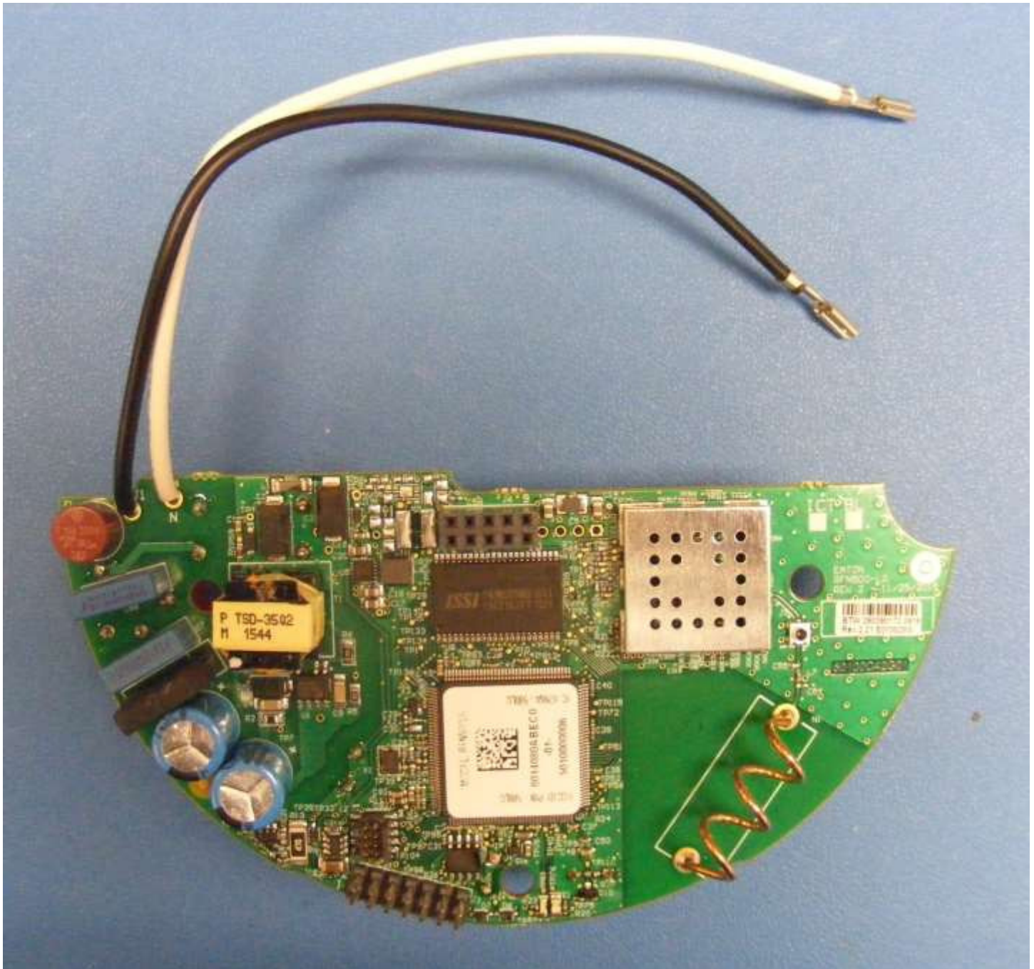
Figure 1: RFN-500LG - Top
