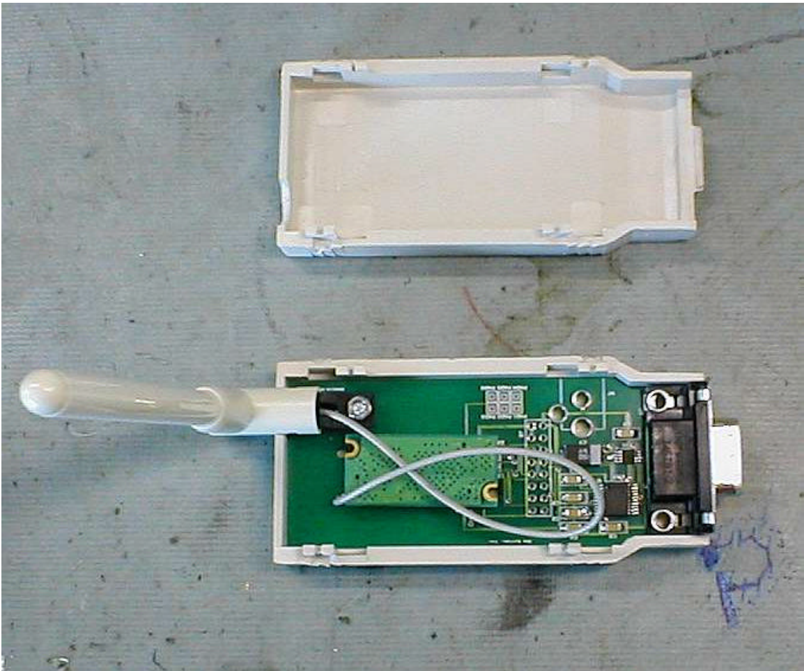
Hub Module Cover Removed
