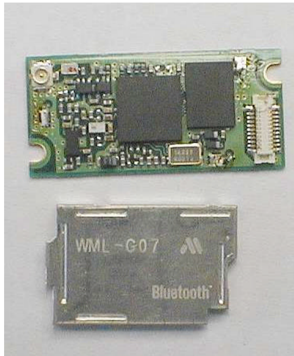
Bluetooth with Shield Removed
