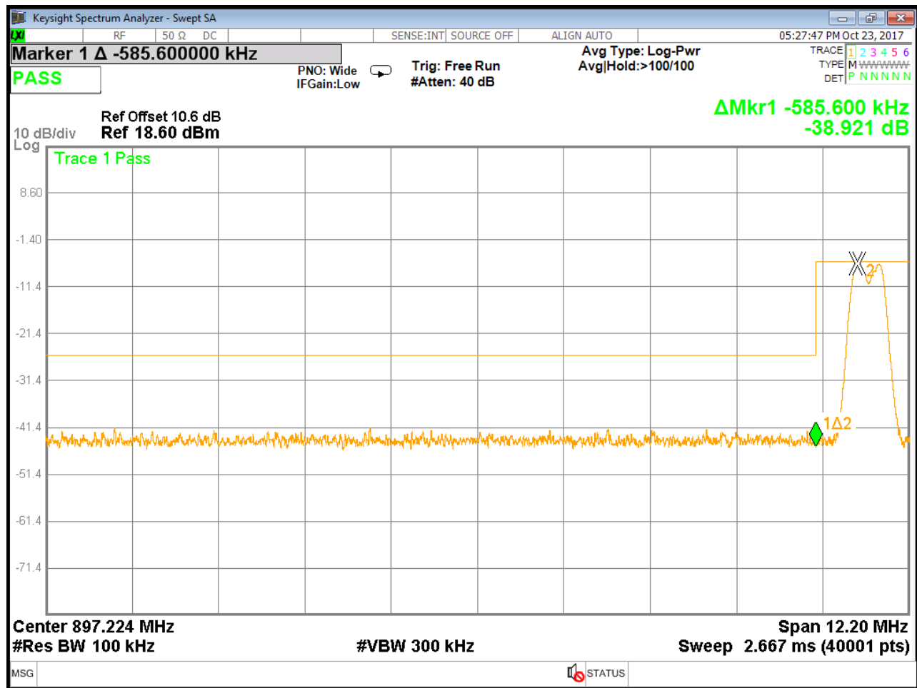
Figure 45: Low Channel (Single Hop), Band-edge, Low Power Setting
