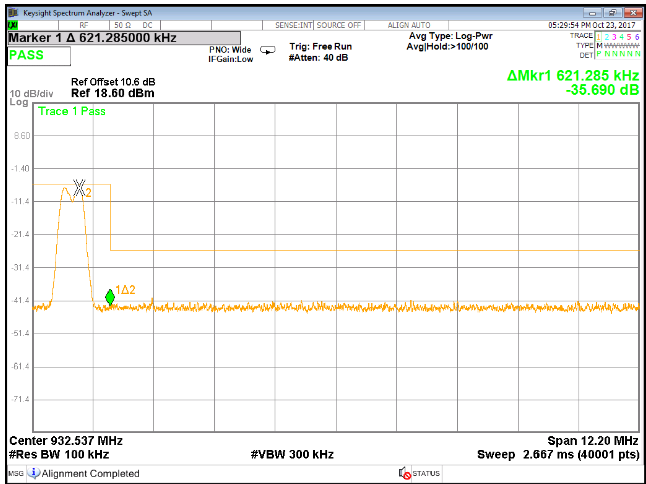
Figure 46: High Channel (Single Hop), Band-edge, Low Power Setting
