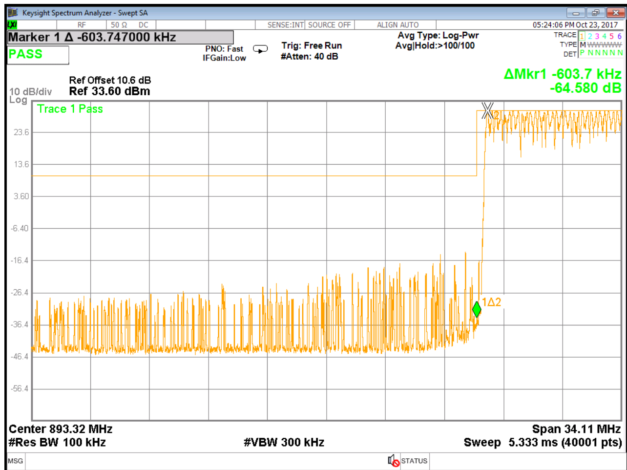
Figure 39: Lower Band-edge, High Power Setting
