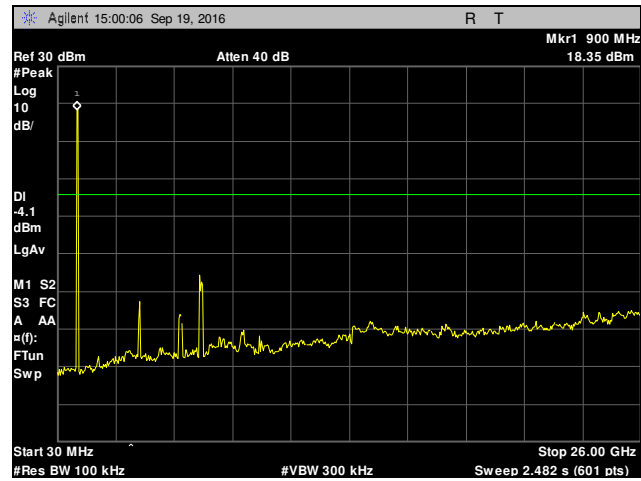
Plot 35. Conducted Spurious Emissions, Hopping
