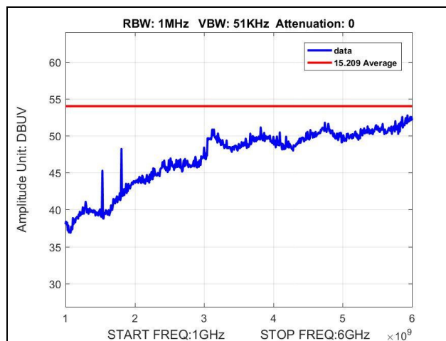
Plot 13. Radiated Spurious Emissions, 1 GHz – 6 GHz, Low Channel, Average
