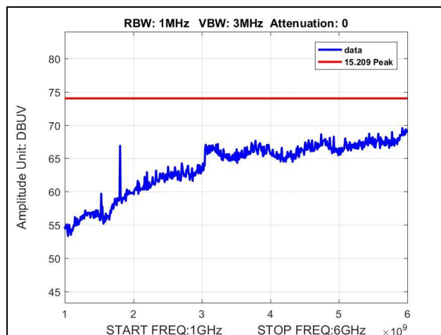
Plot 14. Radiated Spurious Emissions, 1 GHz – 6 GHz, Low Channel, Peak
