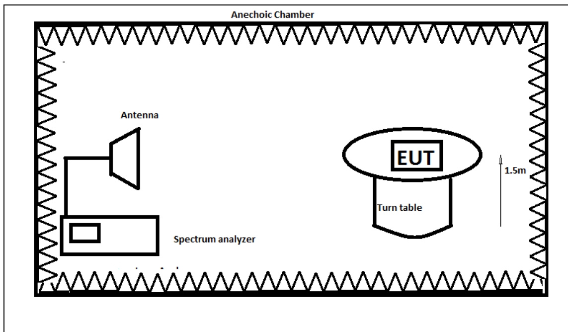
Figure 4. Radiated Spurious Emissions, Test Setup, Above 1 GHz
