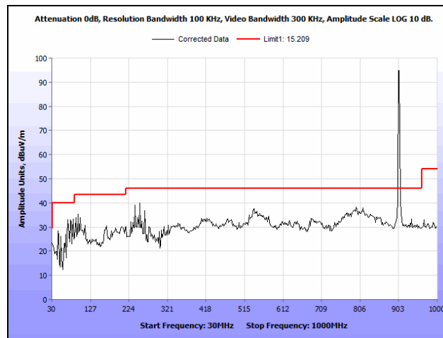
Plot 12. Radiated Spurious Emissions, 30 MHz – 1 GHz, Low Channel
