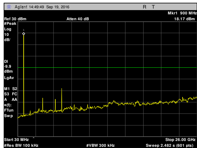
Plot 33. Conducted Spurious Emissions, Mid Channel
