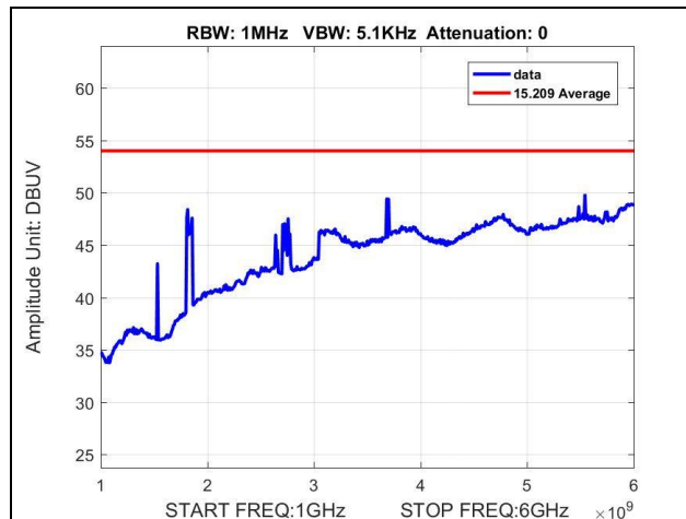
Plot 28. Radiated Spurious Emissions, 1 GHz – 6 GHz, Hopping, Average
