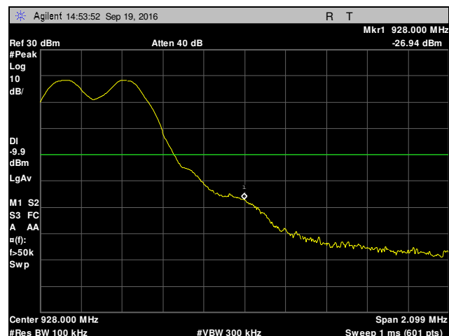
Plot 38. Conducted Band Edge, High Channel
