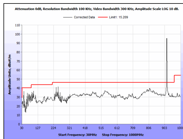
Plot 17. Radiated Spurious Emissions, 30 MHz – 1 GHz, Mid Channel
