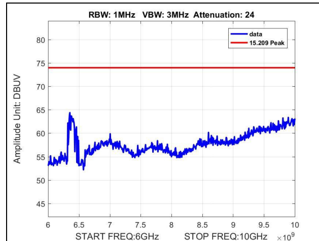
Plot 31. Radiated Spurious Emissions, 6 GHz – 10 GHz, Hopping, Peak
