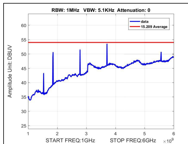
Plot 23. Radiated Spurious Emissions, 1 GHz – 6 GHz, High Channel, Average
