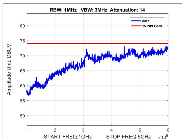
Plot 29. Radiated Spurious Emissions, 1 GHz – 6 GHz, Hopping, Peak
