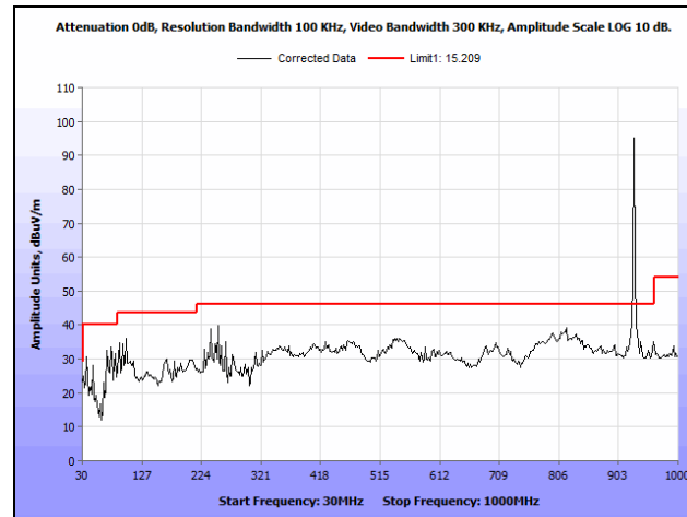
Plot 22. Radiated Spurious Emissions, 30 MHz – 1 GHz, High Channel
