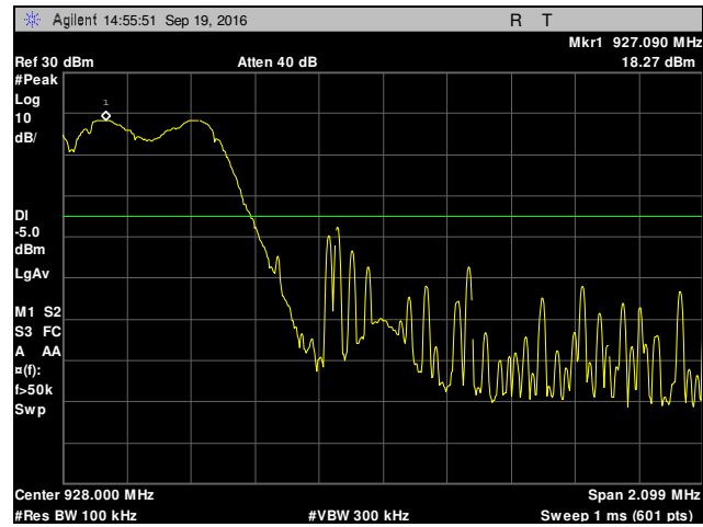
Plot 39. Conducted Band Edge, High Channel, Hopping
