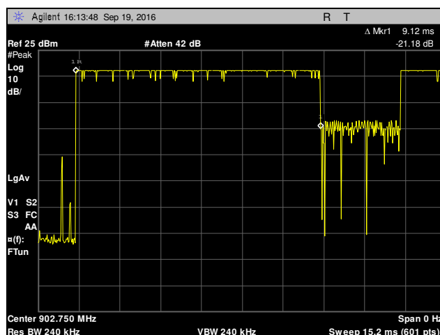
Plot 5. Dwell Time, On Time
