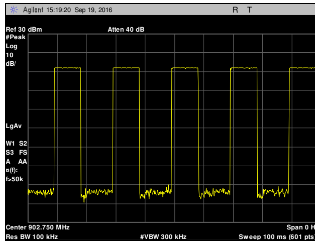
Plot 40. Duty Cycle, 100ms
