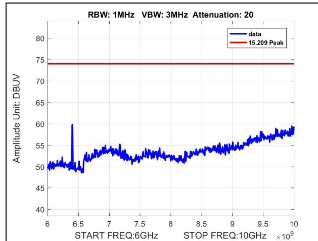
Plot 21. Radiated Spurious Emissions, 6 GHz – 10 GHz, Mid Channel, Peak
