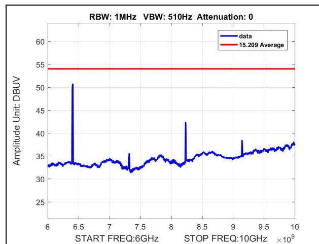
Plot 20. Radiated Spurious Emissions, 6 GHz – 10 GHz, Mid Channel, Average
