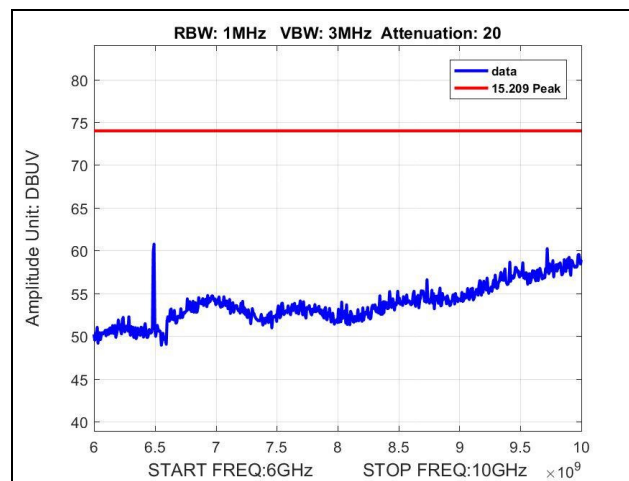
Plot 26. Radiated Spurious Emissions, 6 GHz – 10 GHz, High Channel, Peak
