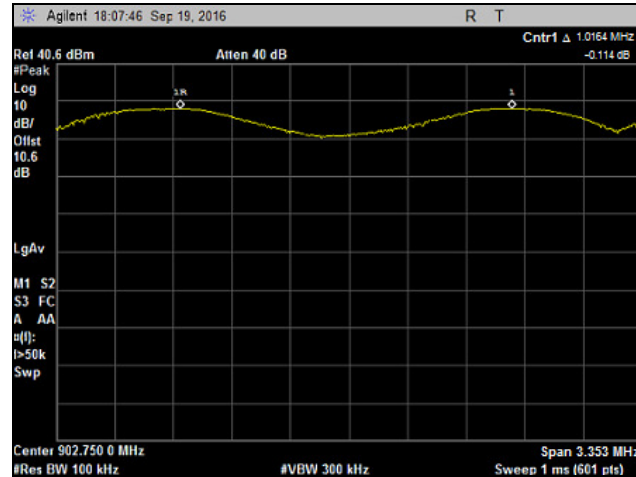
Plot 8. Channel Separation
