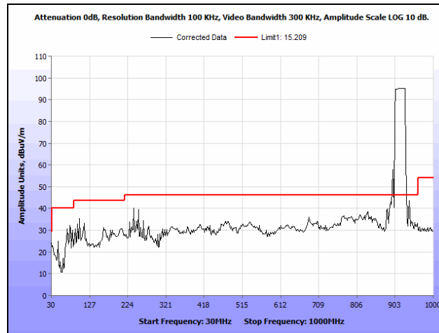
Plot 27. Radiated Spurious Emissions, 30 MHz – 1 GHz, Hopping
