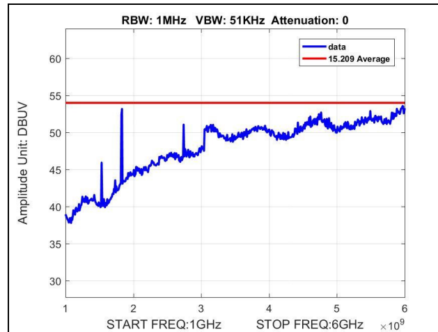
Plot 18. Radiated Spurious Emissions, 1 GHz – 6 GHz, Mid Channel, Average
