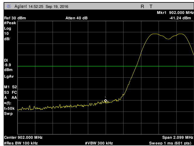
Plot 36. Conducted Band Edge, Low Channel
