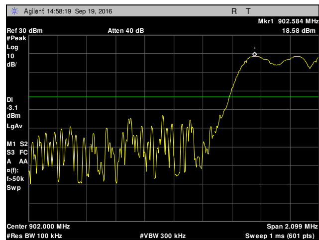
Plot 37. Conducted Band Edge, Low Channel, Hopping
