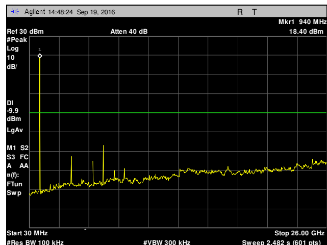
Plot 34. Conducted Spurious Emissions, High Channel
