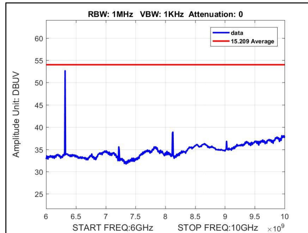
Plot 15. Radiated Spurious Emissions, 6 GHz – 10 GHz, Low Channel, Average
