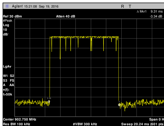
Plot 41. Duty Cycle, On Time
