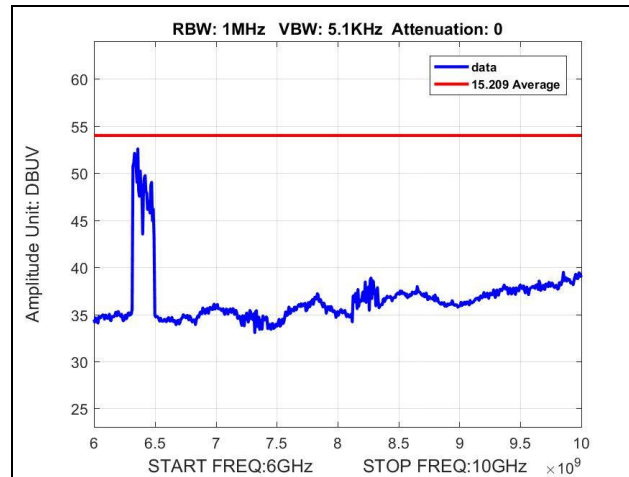
Plot 30. Radiated Spurious Emissions, 6 GHz – 10 GHz, Hopping, Average
