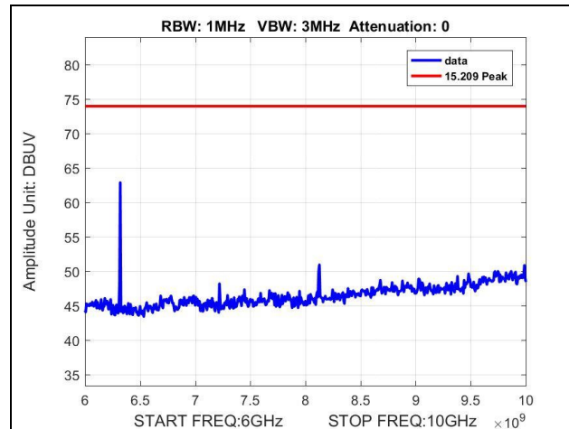
Plot 16. Radiated Spurious Emissions, 6 GHz – 10 GHz, Low Channel, Peak
