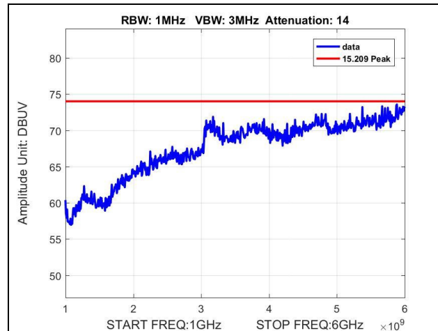
Plot 19. Radiated Spurious Emissions, 1 GHz – 6 GHz, Mid Channel, Peak
