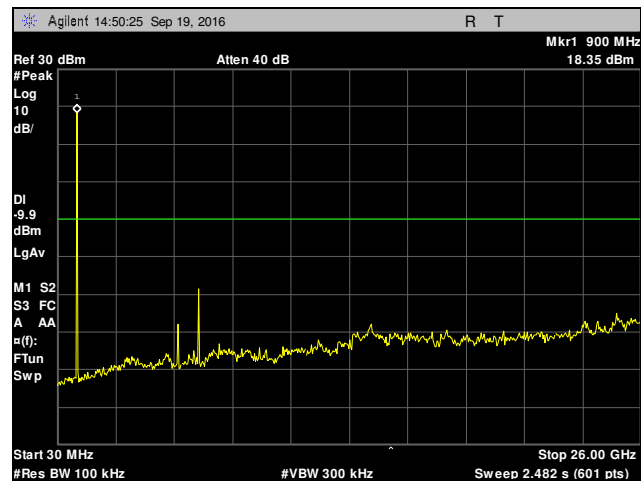
Plot 32. Conducted Spurious Emissions, Low Channel
