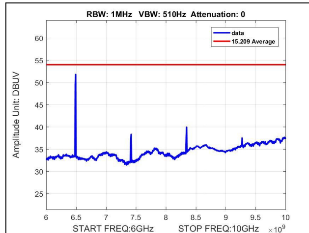
Plot 25. Radiated Spurious Emissions, 6 GHz – 10 GHz, High Channel, Average
