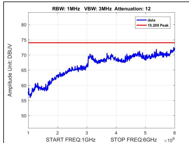
Plot 24. Radiated Spurious Emissions, 1 GHz – 6 GHz, High Channel, Peak
