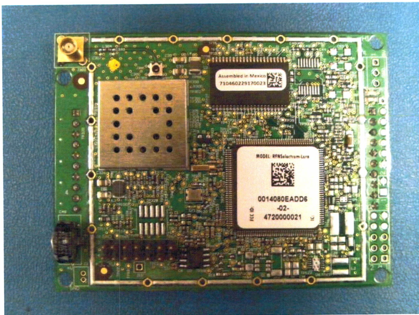
Figure 1: RFN SelectComm 1272 (3.3V) - Top
