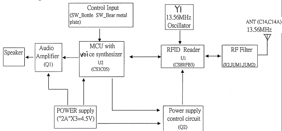
Reader Block Diagram:
