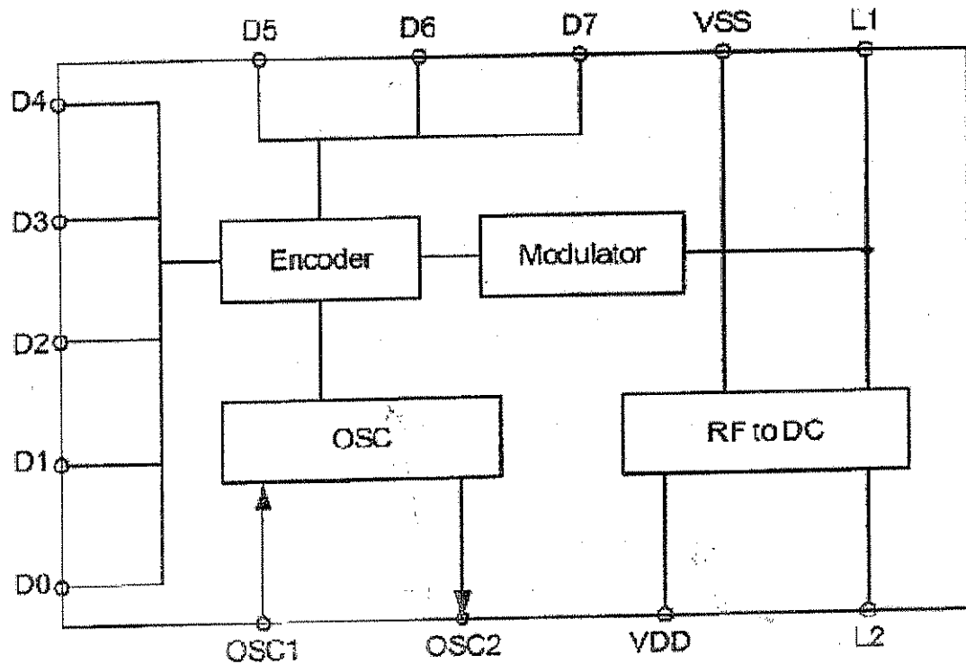
Block Diagram
