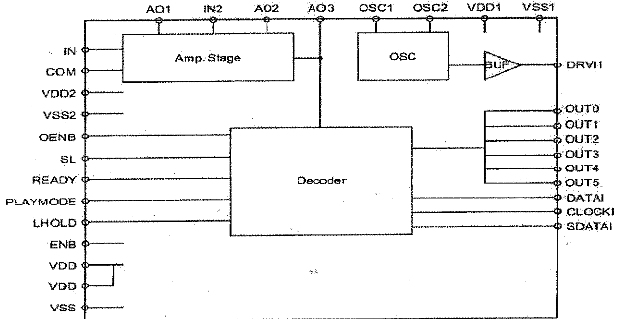
Block Diagram
