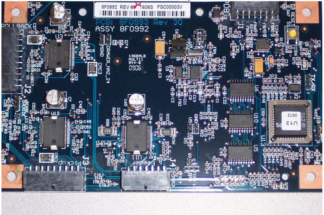
6800 Transmitter Board Bottom
