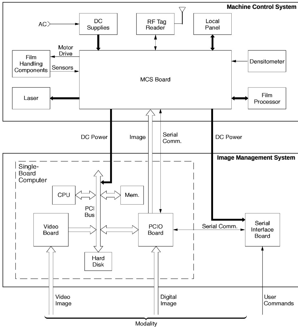
DryView 8100 Laser Imager Block Diagram
