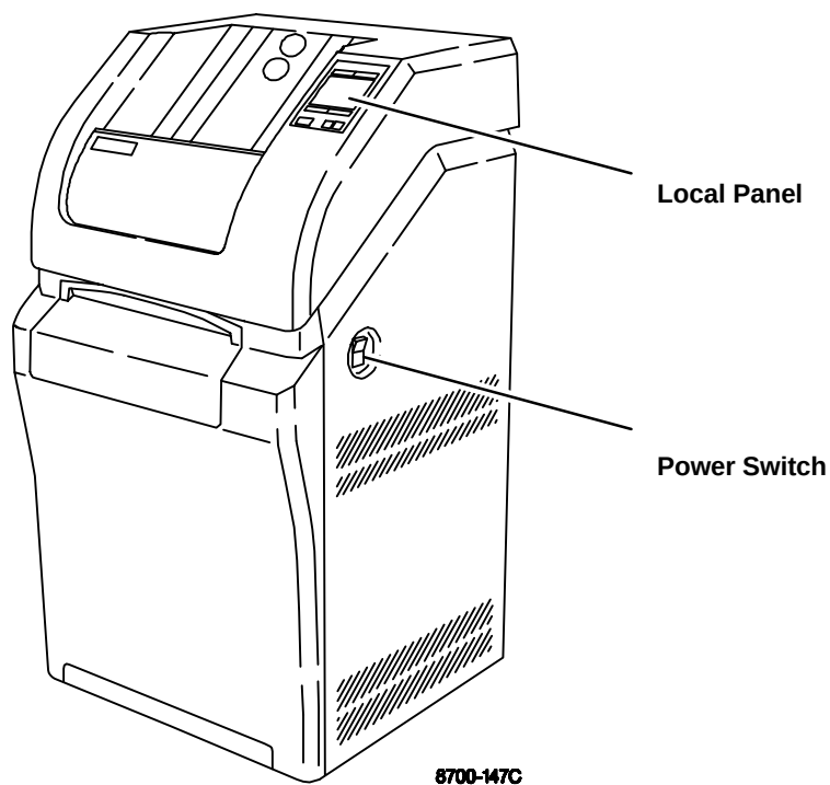
Figure 3-1. Power Switch and Local Panel
