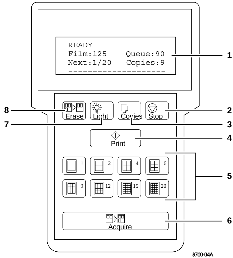
Figure 2-7. DryView 8700/8500 Keypad
