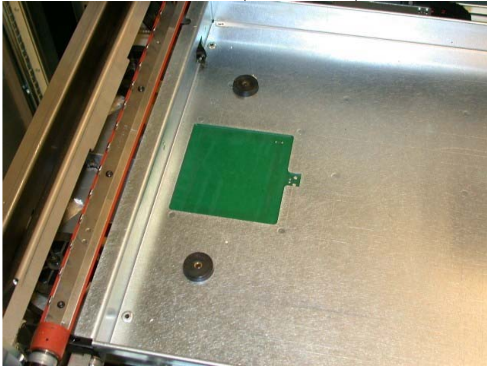
Antenna installed in sample host device - top view
