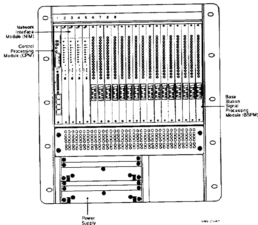
Figure 2-3 Base Station Equipment Shelf
