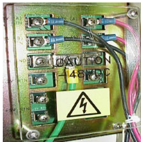
Figure 7 – Detail of Terminal Block
