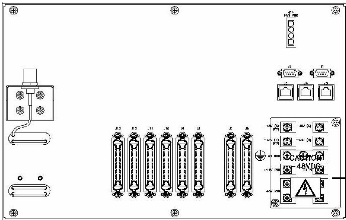
Figure 6 – Host Digital Terminal – Rear View
