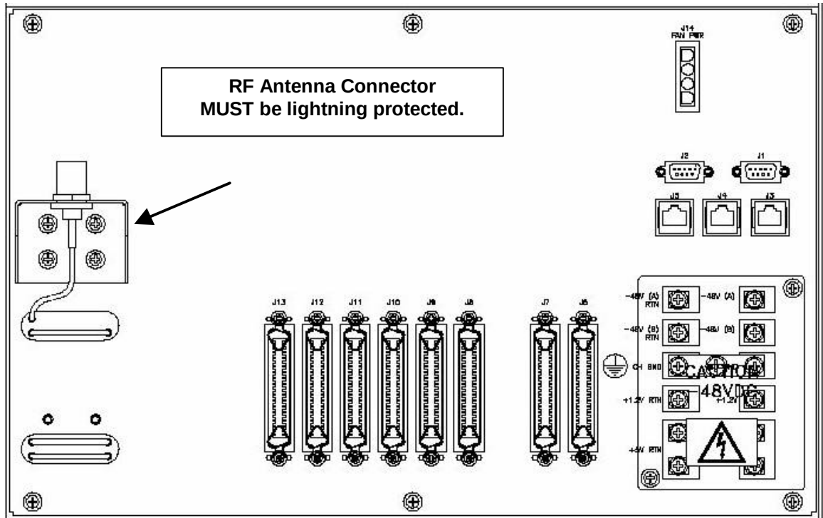
Figure 10 – Location of RF Antenna Connector
