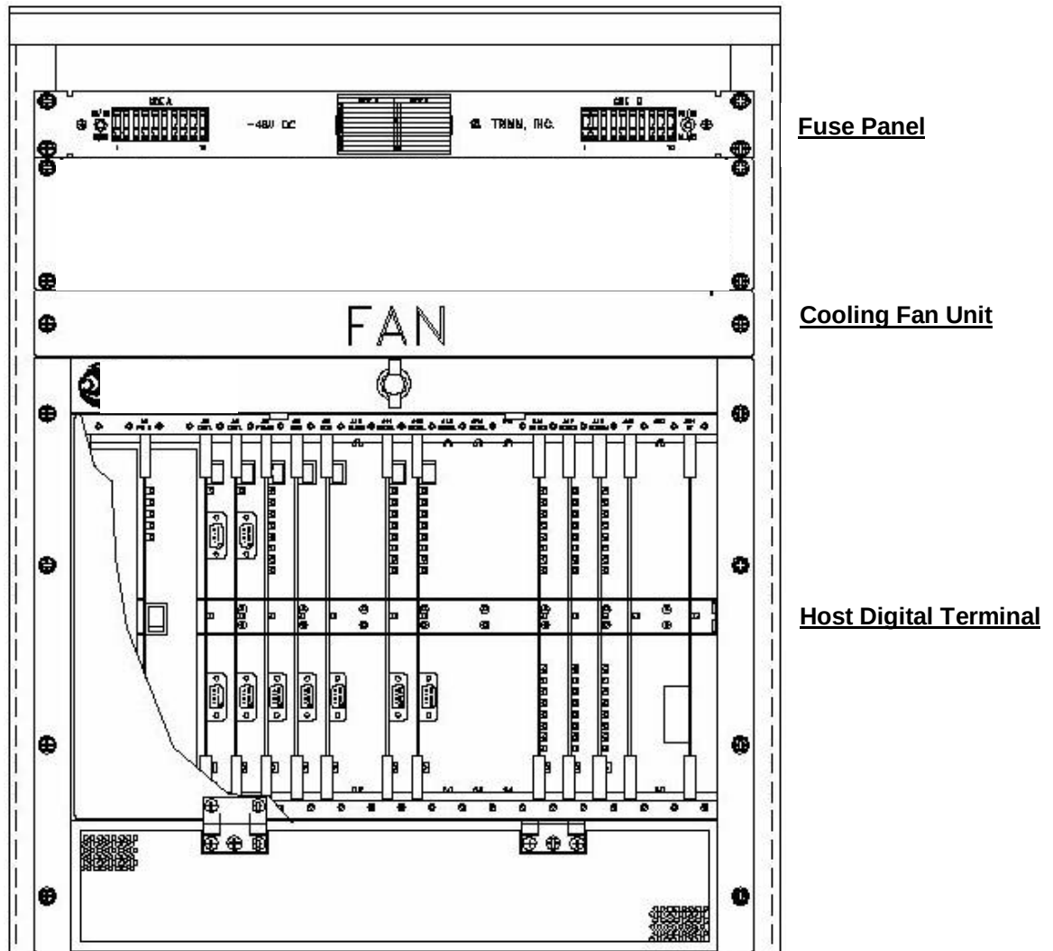
Figure 1 – Rack Assembly
