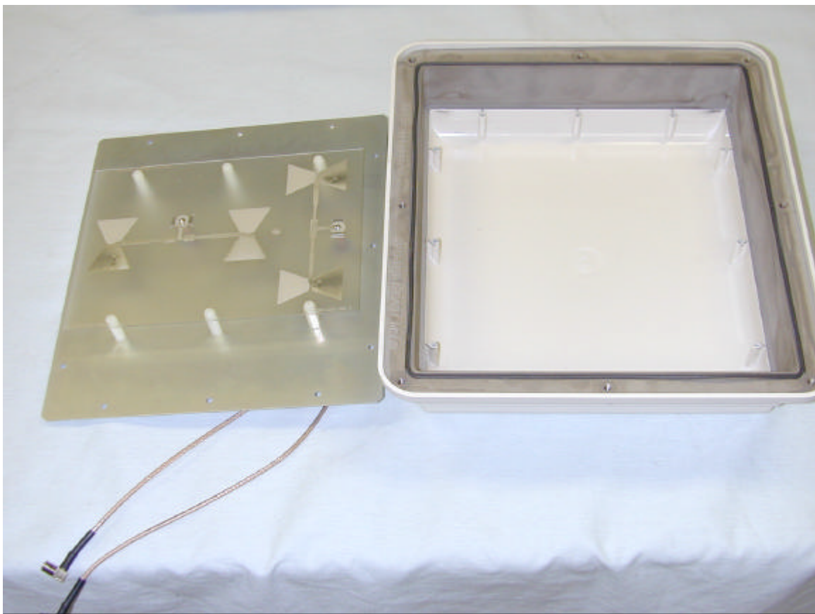
Photo 5 - RU Antenna
