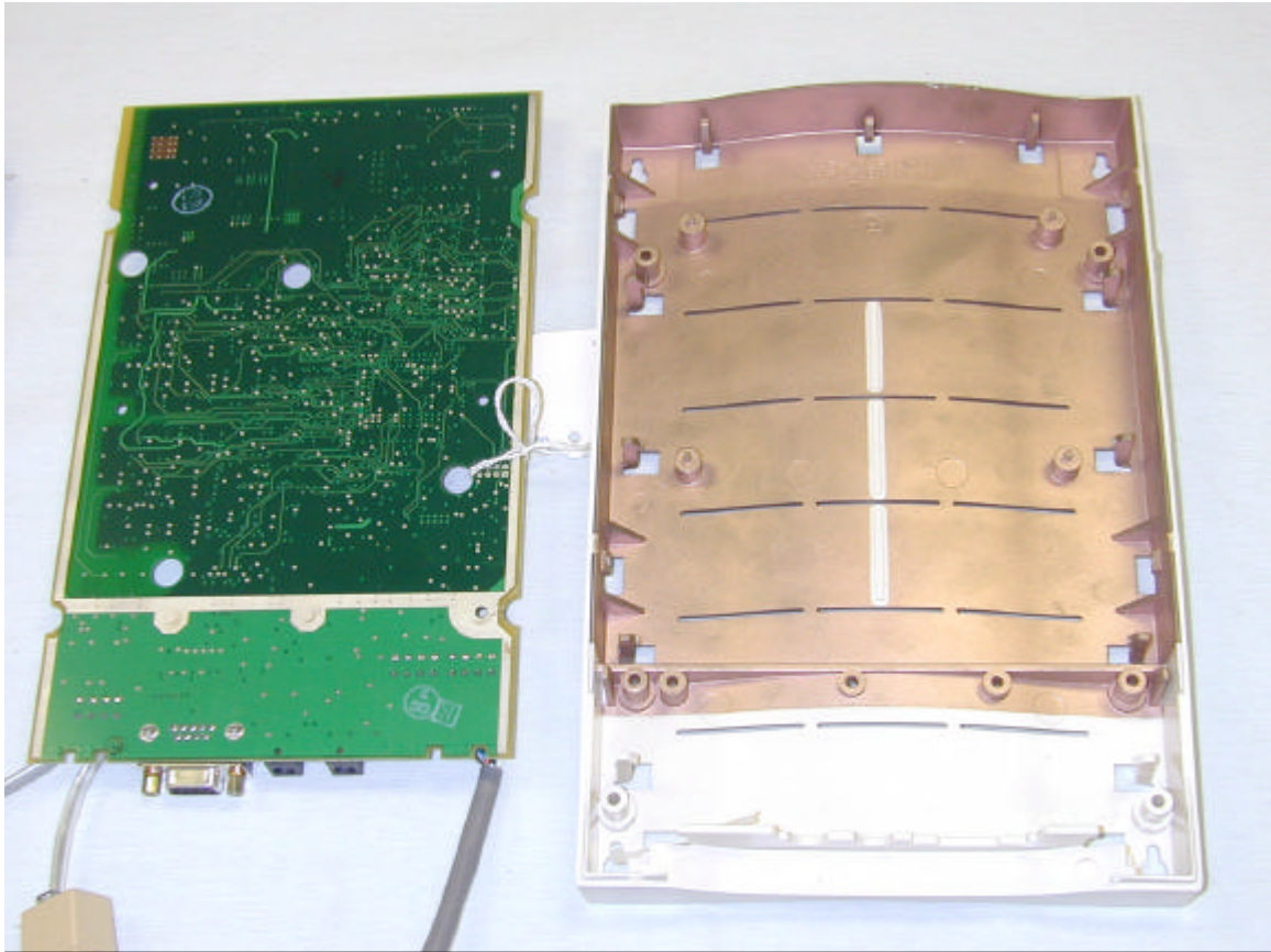
Photo 7 - CPI Bottom
