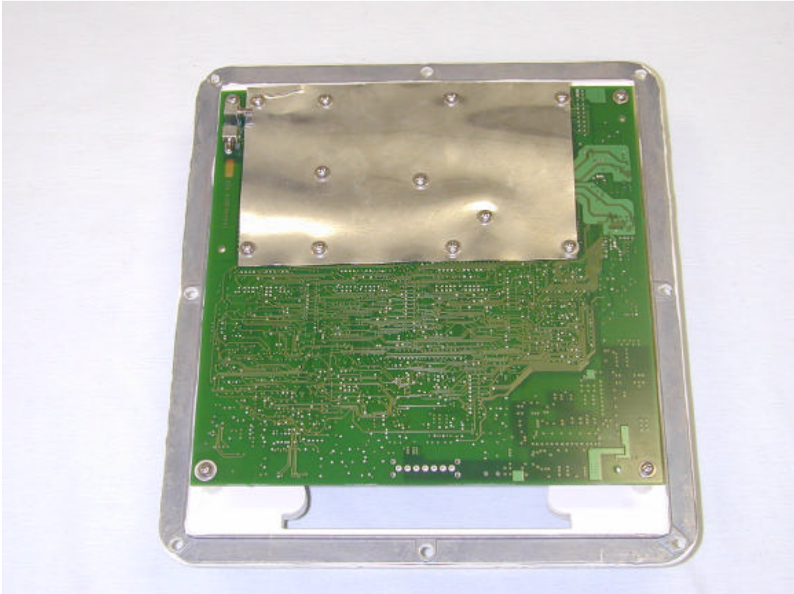
Photo 1 - RU RF board trace side
