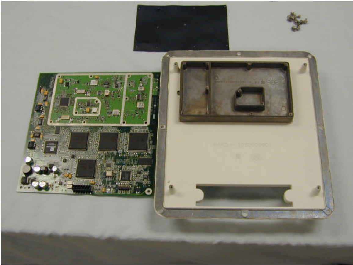
Photo 3 - RU RF Board component side
