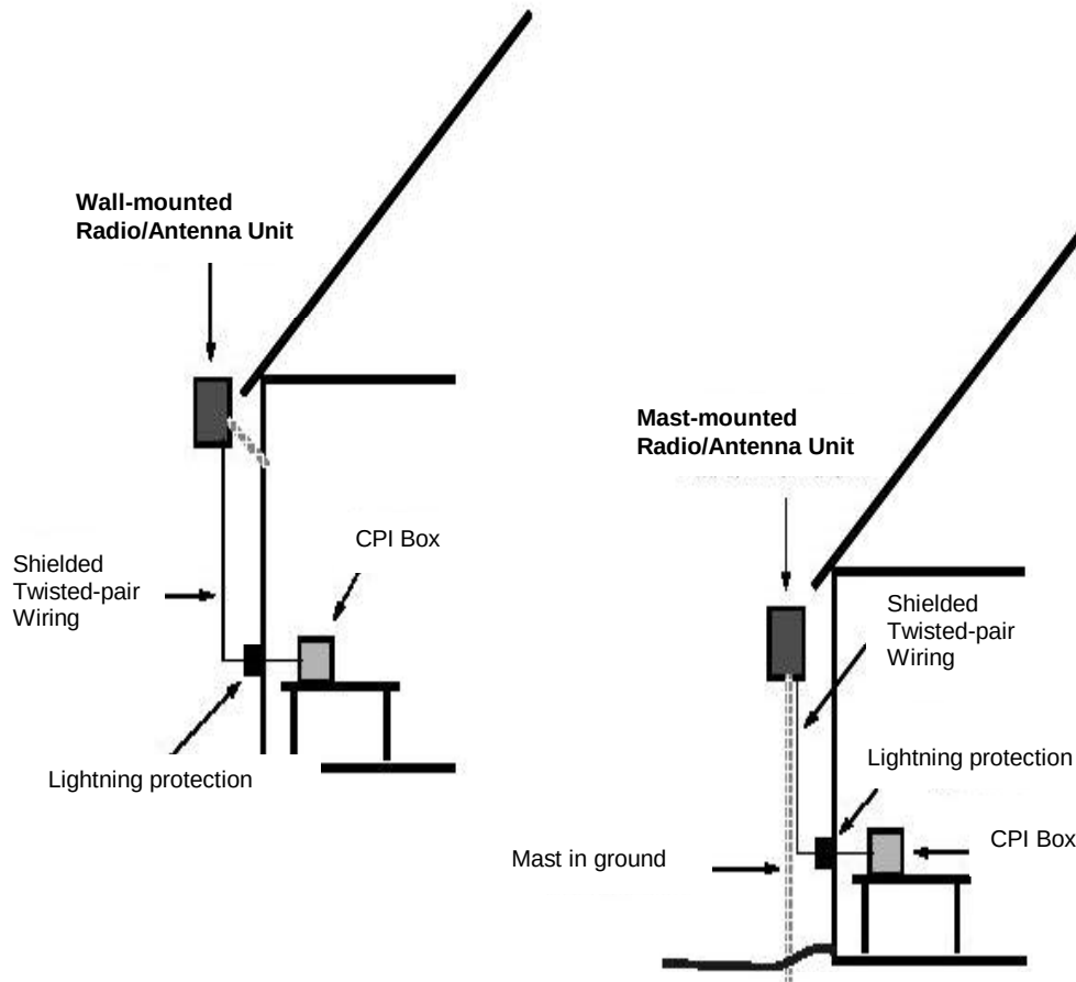
Figure 6 – CPI Installation
