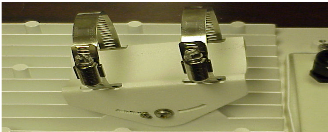
Figure 3 – Vertical Pole Mount Assembly
