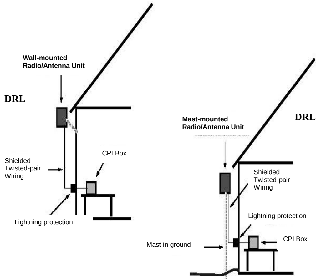
Figure 1 – Typical Installation
