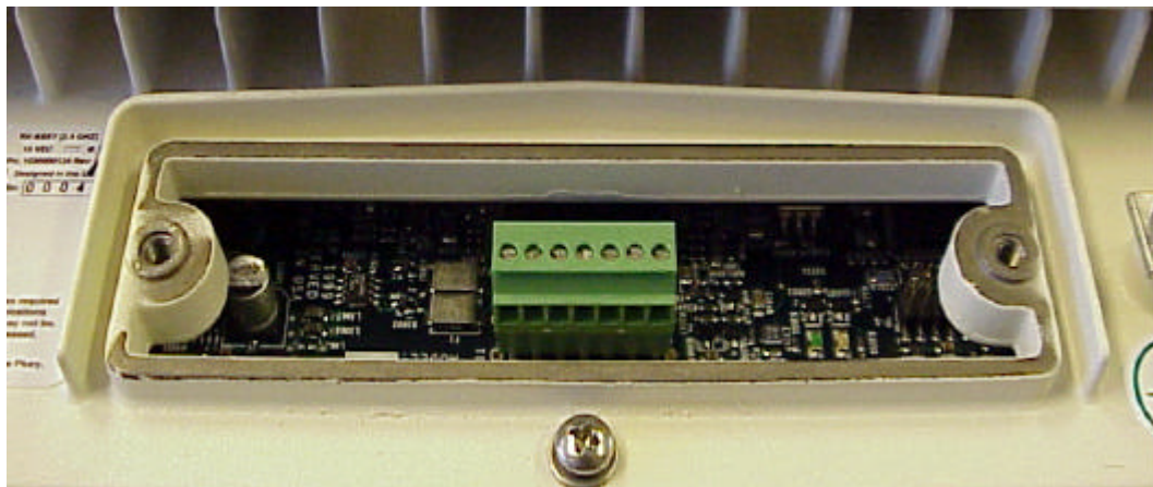
Figure 5 – Terminal Block
