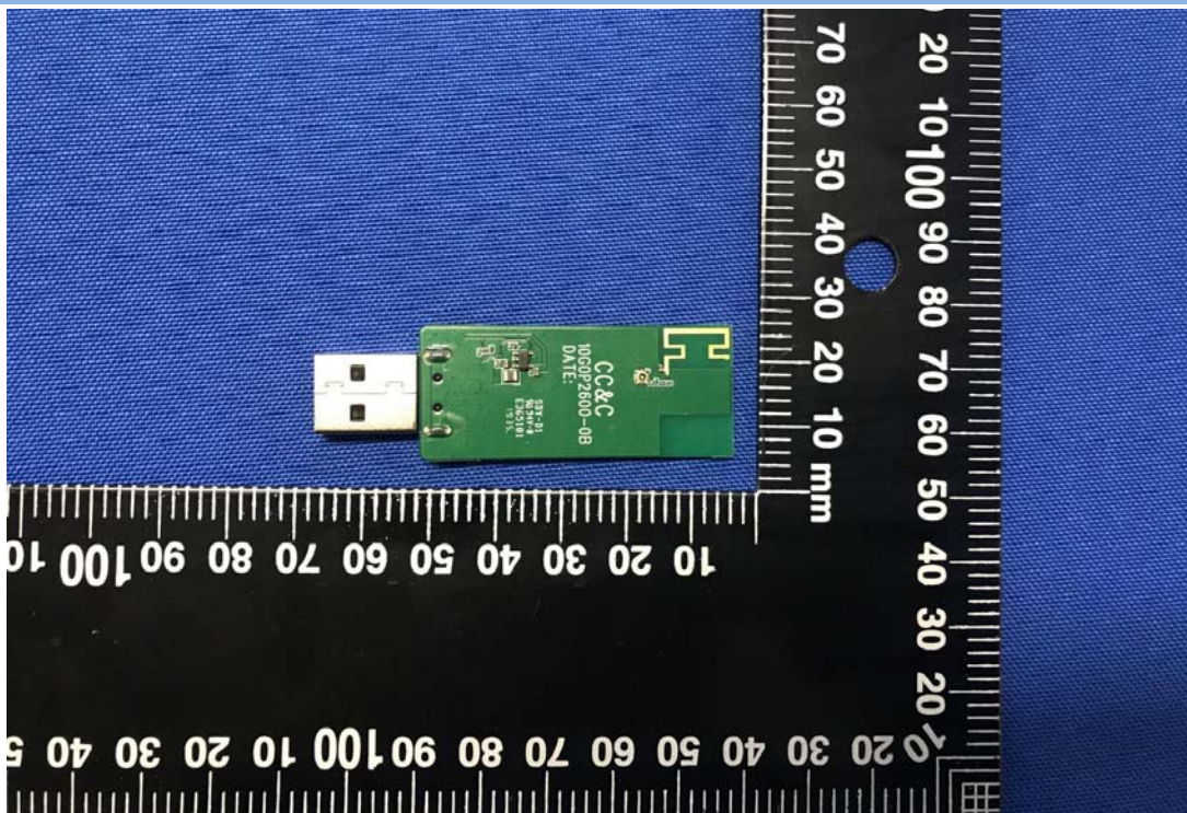
MAIN BOARD REAR VIEW 1
