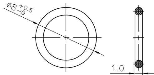
O-ring
